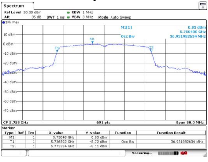
99% Occupied Bandwidth
