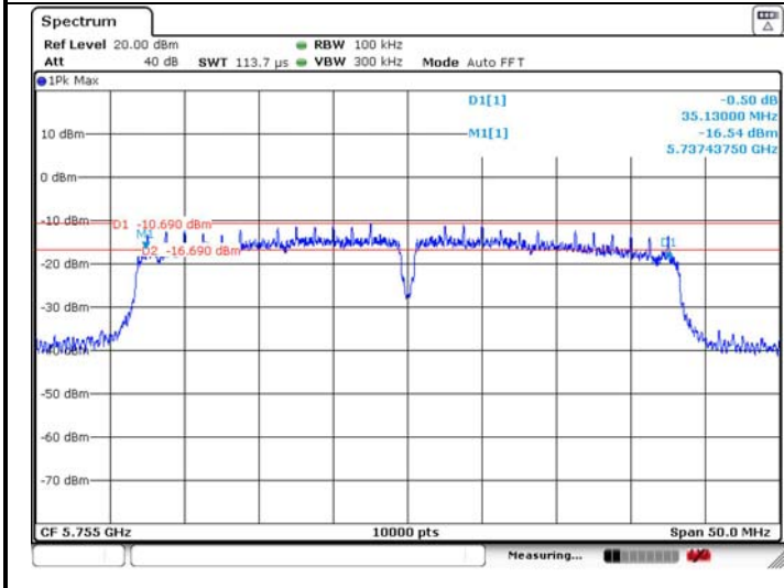
6dB Bandwidth
