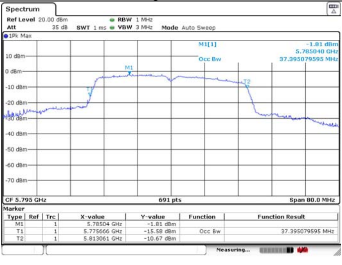
99% Occupied Bandwidth
