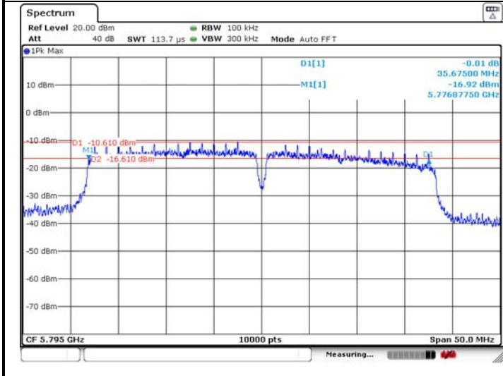
6dB Bandwidth
