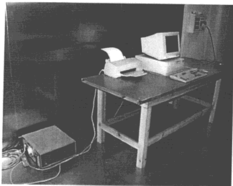
Photograph 7. Conducted disturbance at mains ports emission test
