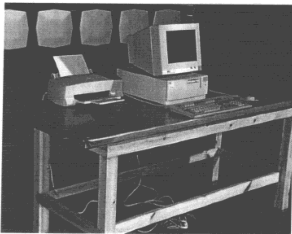
Photograph 2. Radiated disturbance emission test.
