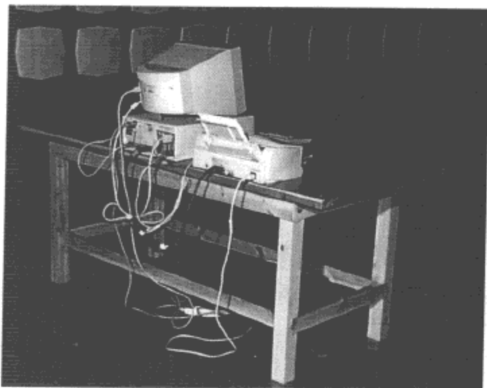
Photograph 3. Radiated disturbance emission test.
