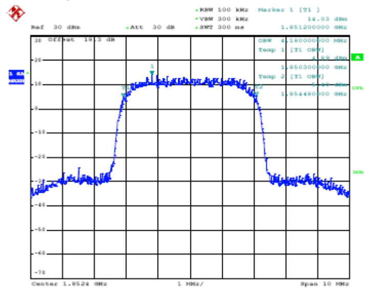
99% Occupied Bandwidth Plot on Channel 9262 (1852.4 MHz)
