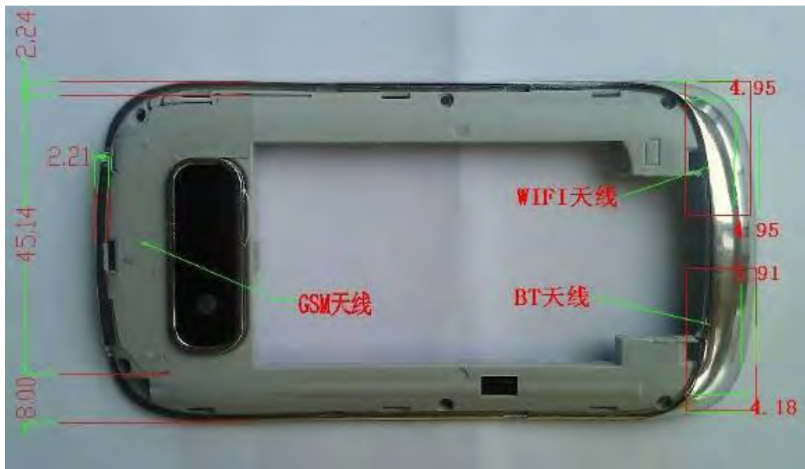
Picture 11.1 Antenna Locations
