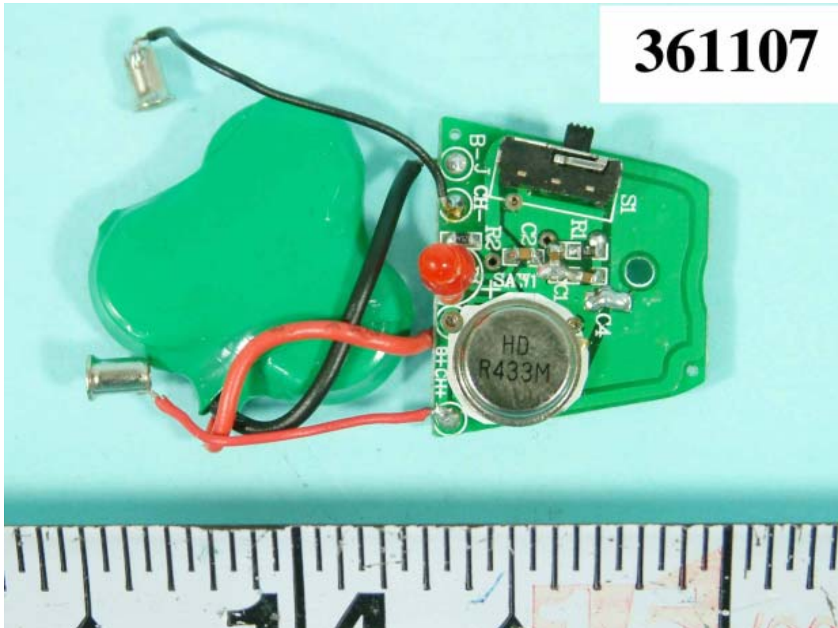
FRONT SIDE OF MAIN BOARD OF EUT
