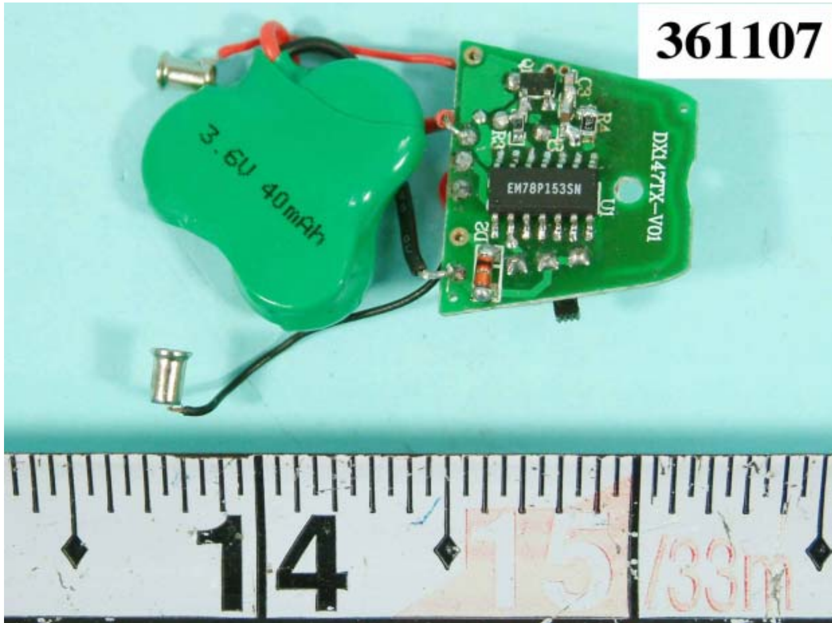
REAR SIDE OF MAIN BOARD OF EUT
