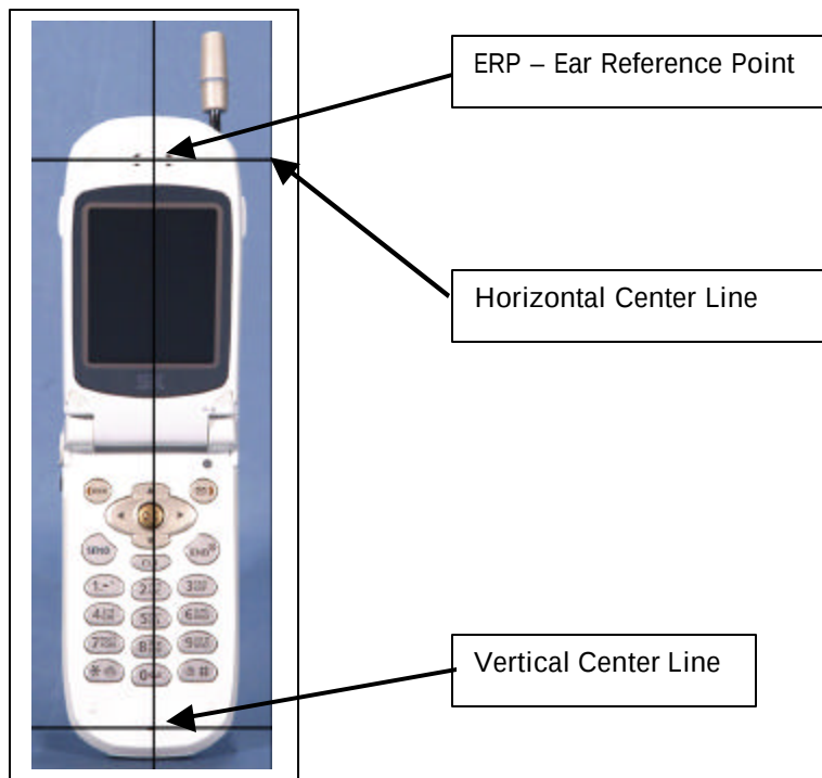
Figure 12.1 Handset Reference Points
