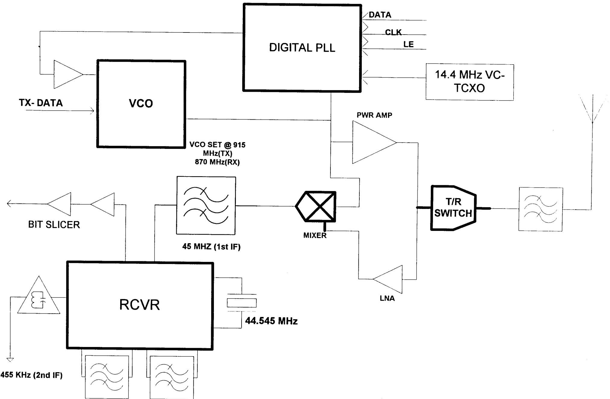
TRANSCEIVER BLK DIAGRAM
