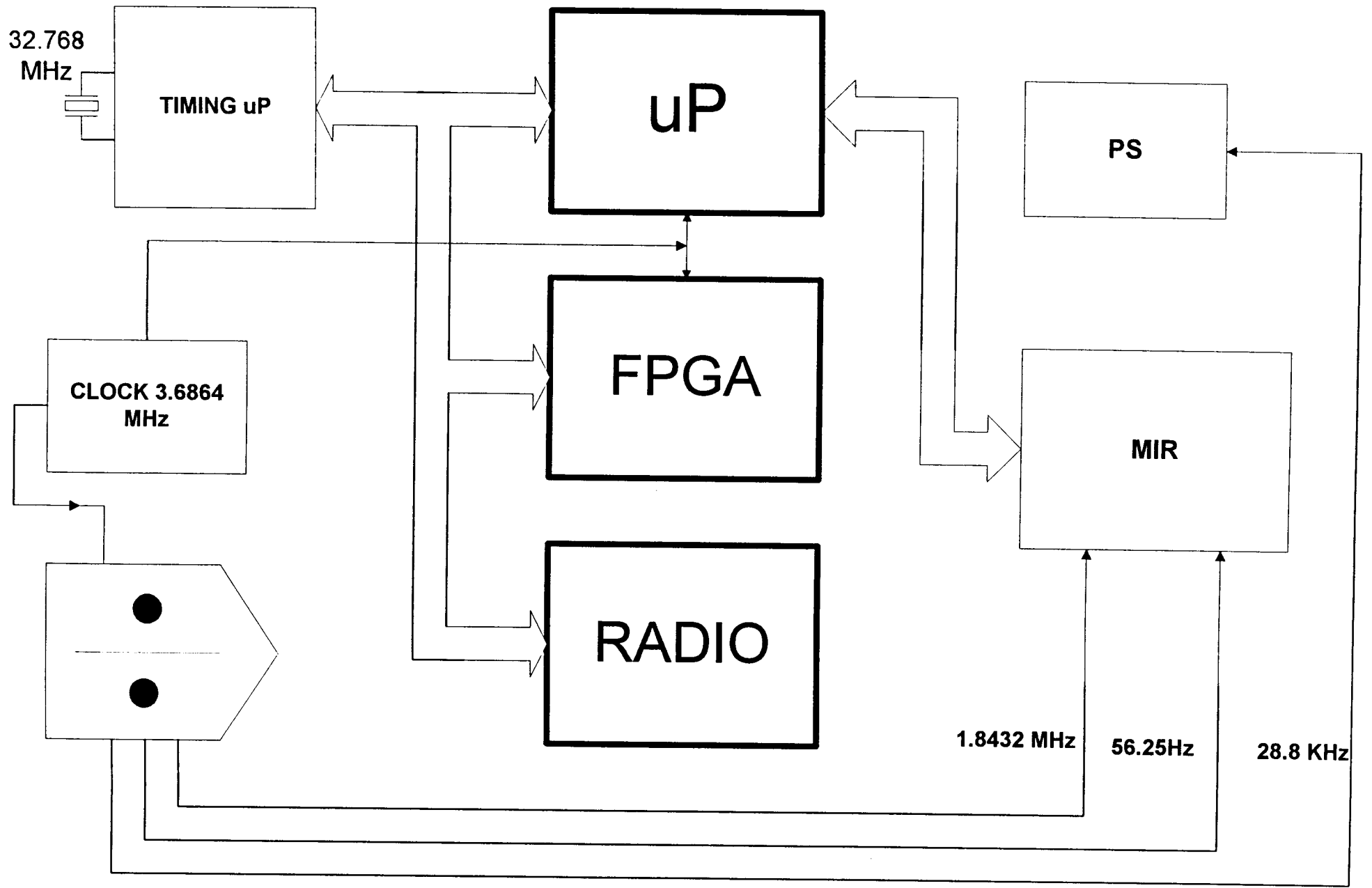
MONITOR BLK DIAGRAM
