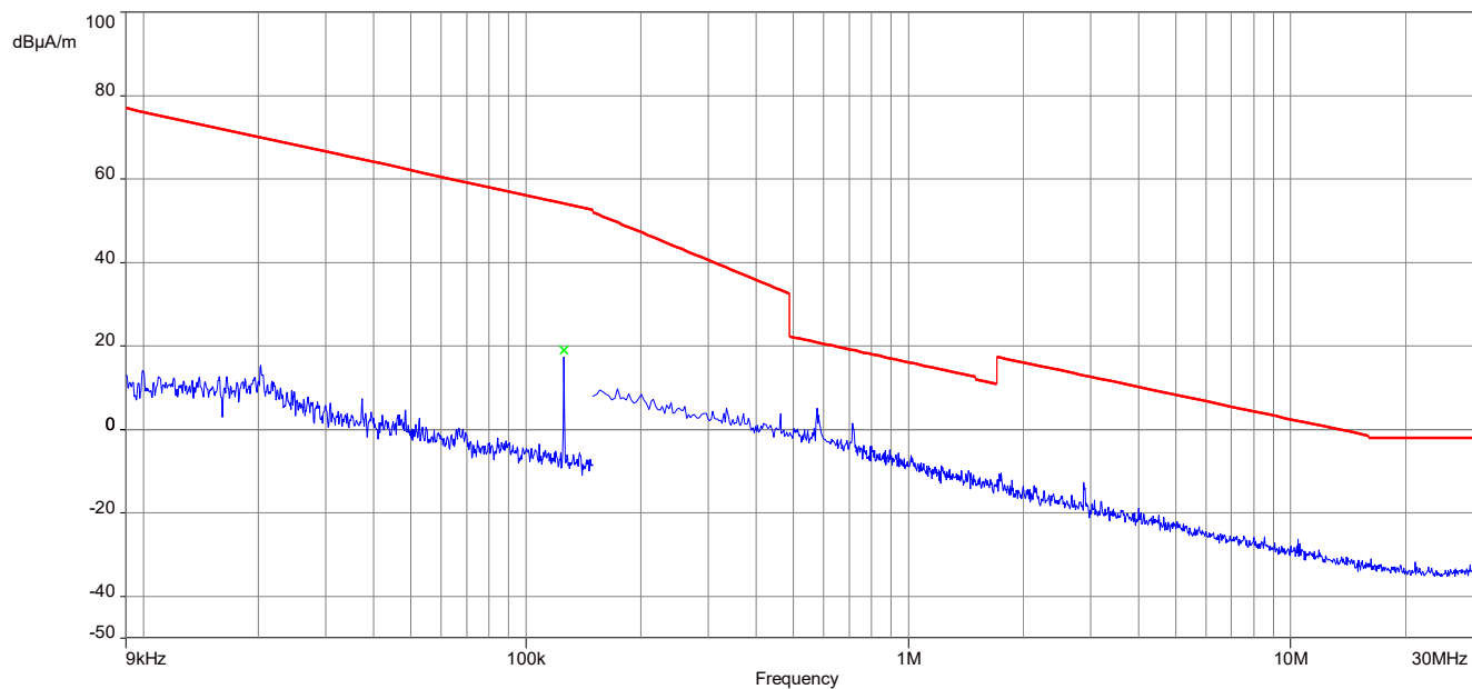
Plot 1: 9 kHz – 30 MHz, magnetic spurious emissions IC
