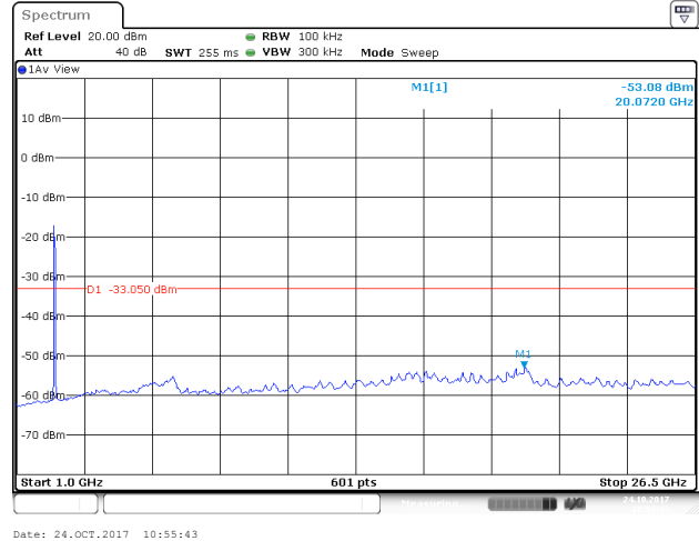
802.11 n40 on channel 06
