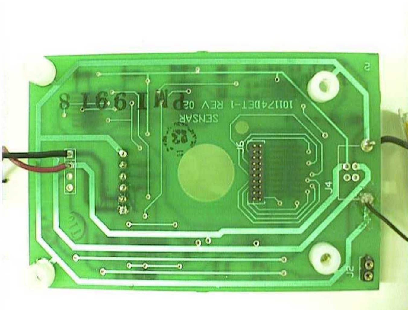
Camera Interface Board (Side 1)
