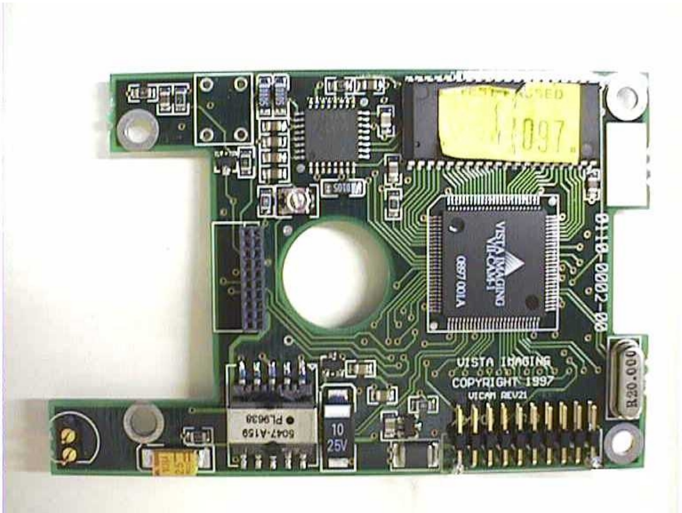
ViCam Parallel Camera Board (Side 1)
