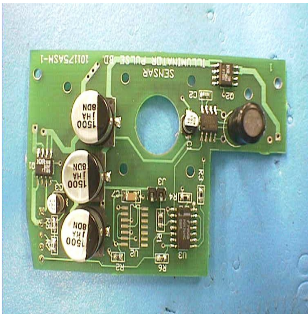
Illuminator Pulse Board (Side 1)
