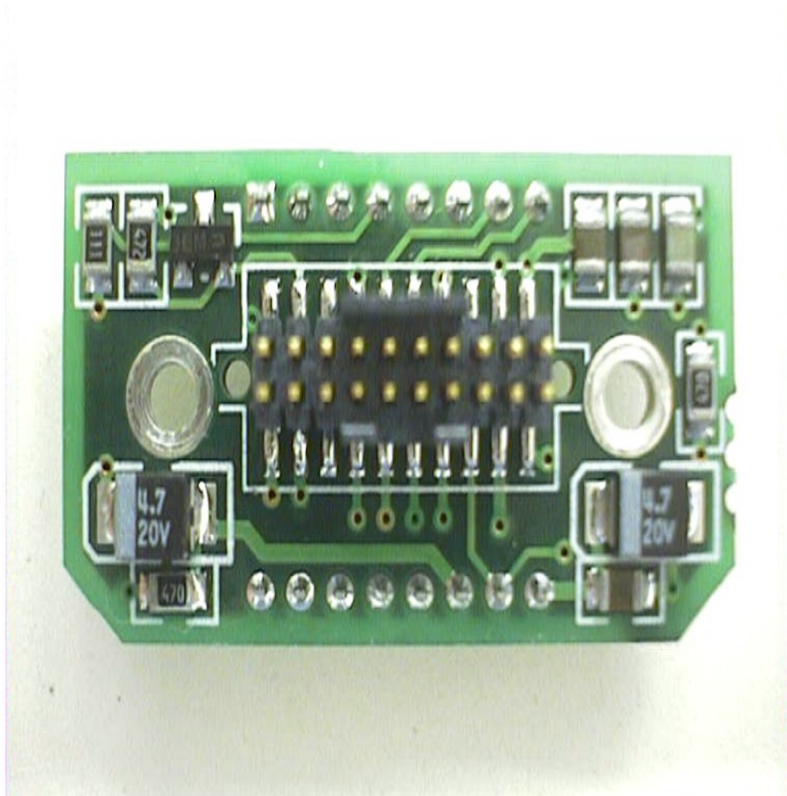
Photo 9: ViCam CCD Sensor Board (Side 1)
