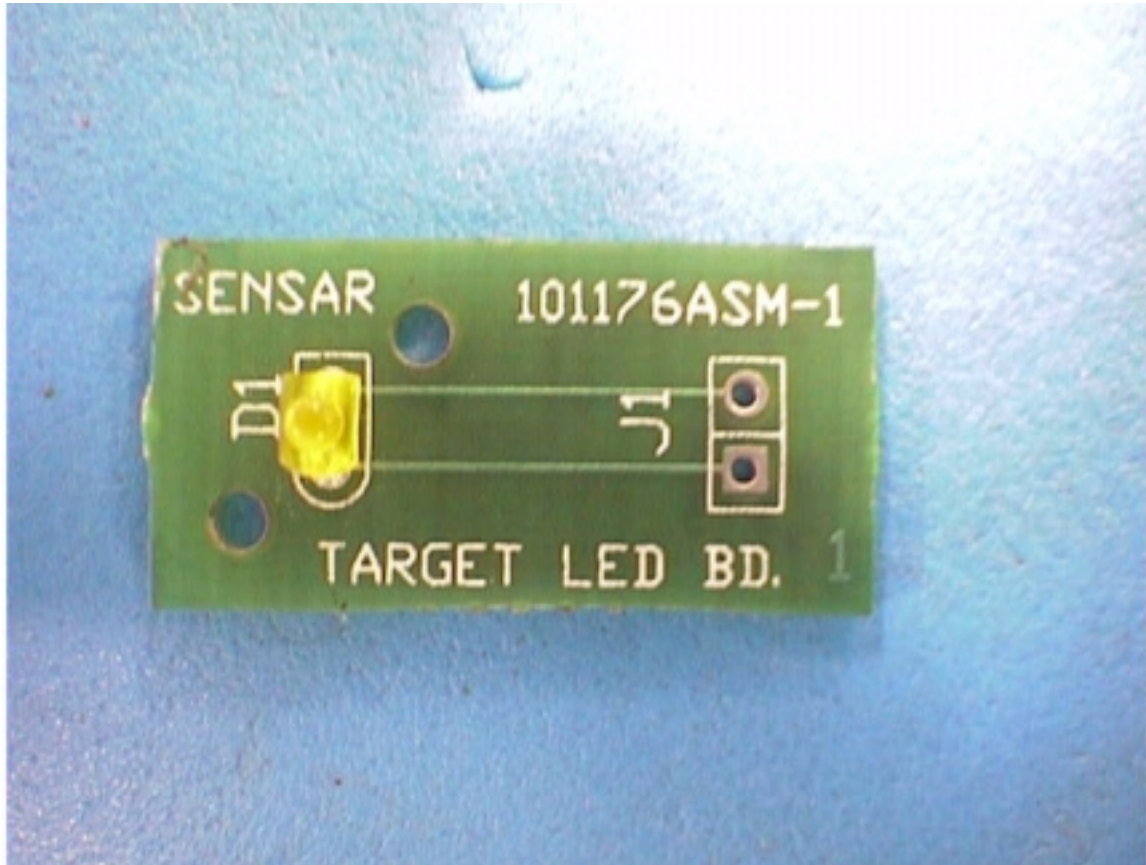
Photo 5: Target LED Board (Side 1)
