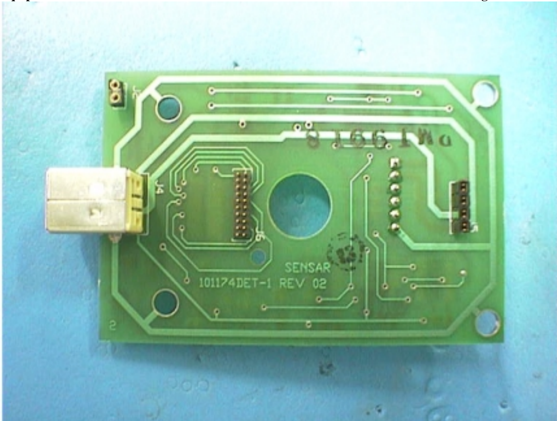
Photo 2: Camera Interface Board (Side 2)
