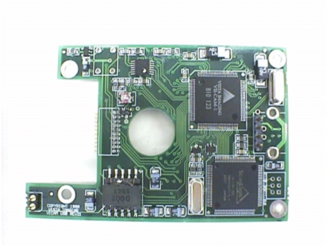
Photo 7: ViCam Parallel Camera Board (Side 1)
