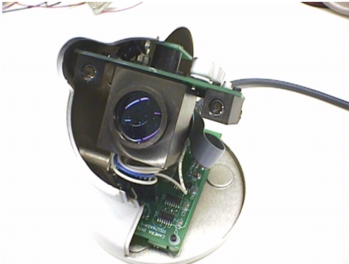
Internal Chassis and Board mounting Photo 3
