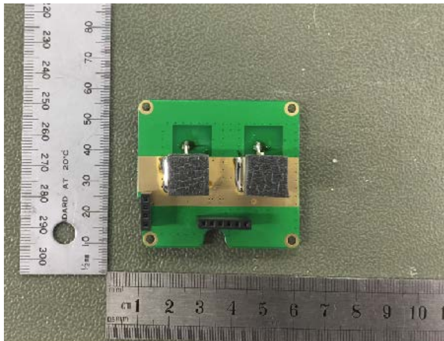
Figure 19. Exciter VCO PCB Bottom View.
