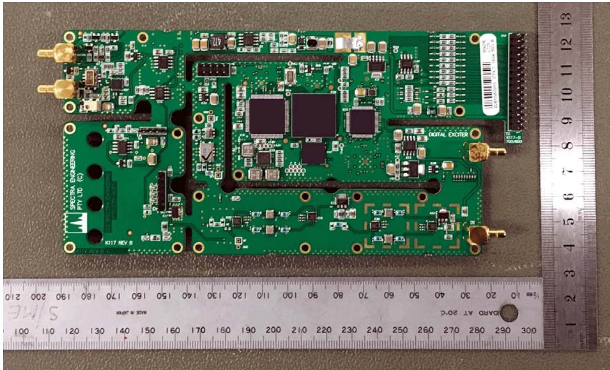
Figure 15. Exciter PCB TOP View.
