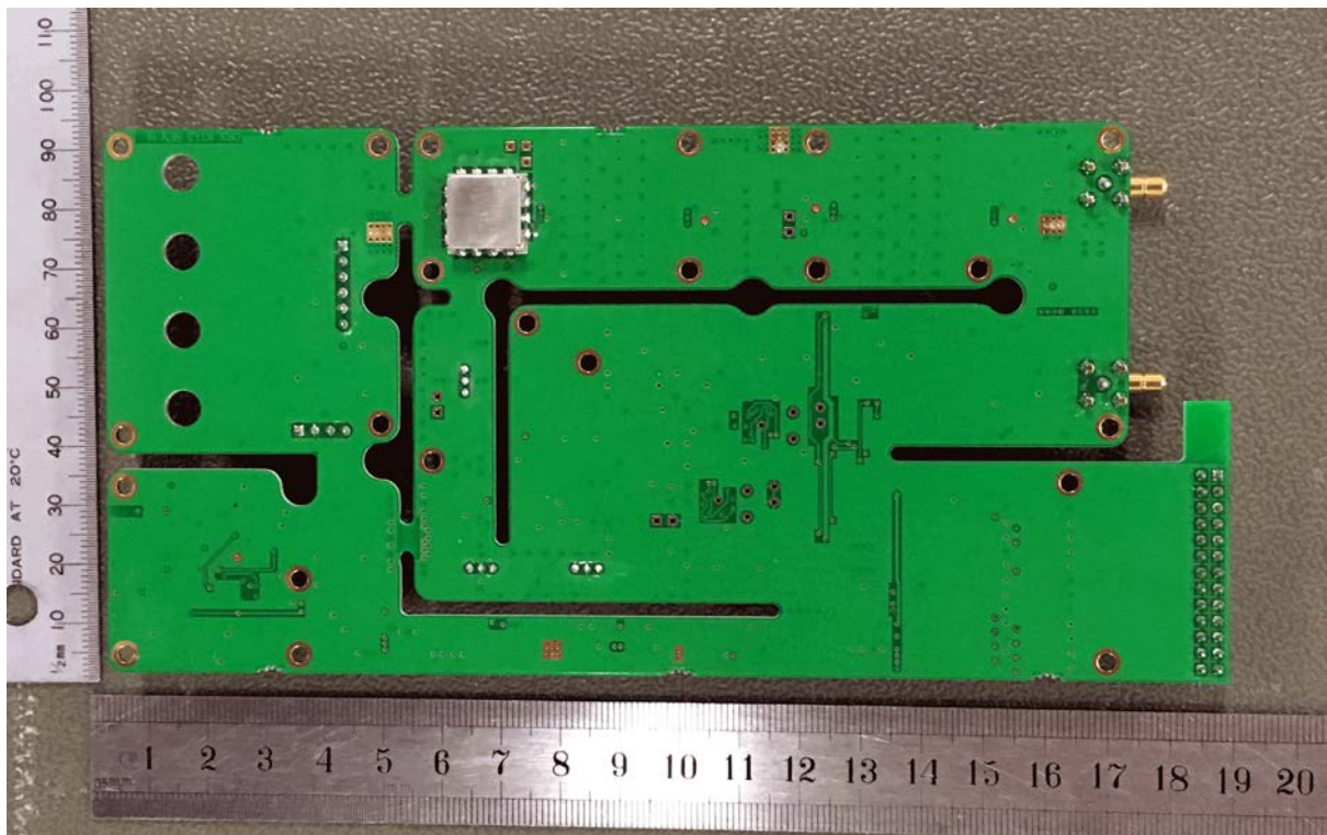
Figure 10. Receiver PCB Bottom View.
