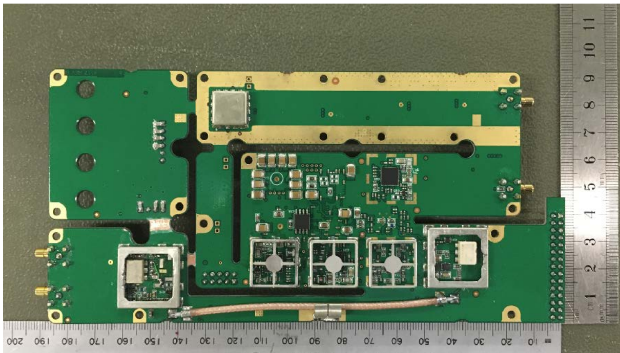
Figure 17. Exciter PCB Bottom View- No shield covers.
