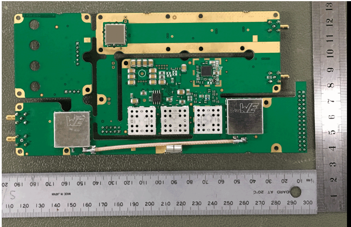
Figure 16. Exciter PCB Bottom View -with Shields.
