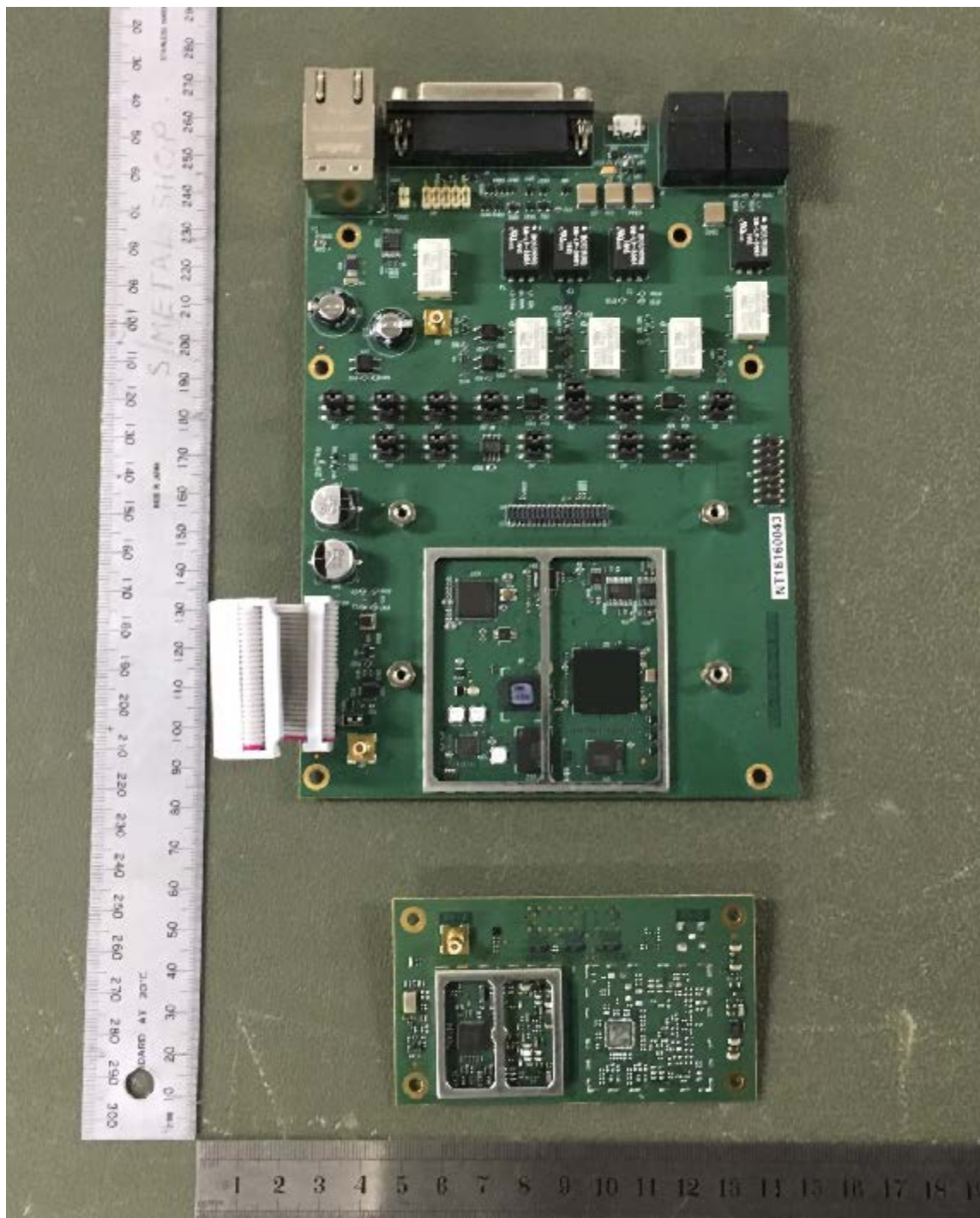
Figure 26. DSP Logic Board- Without Shields.
