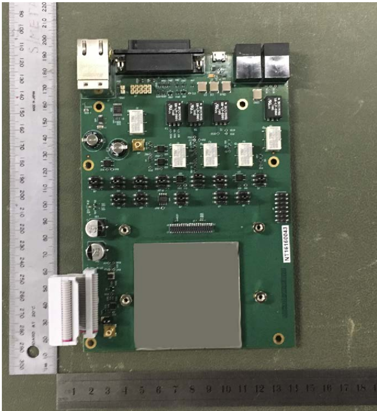
Figure 22. DSP Logic Board Top View.
