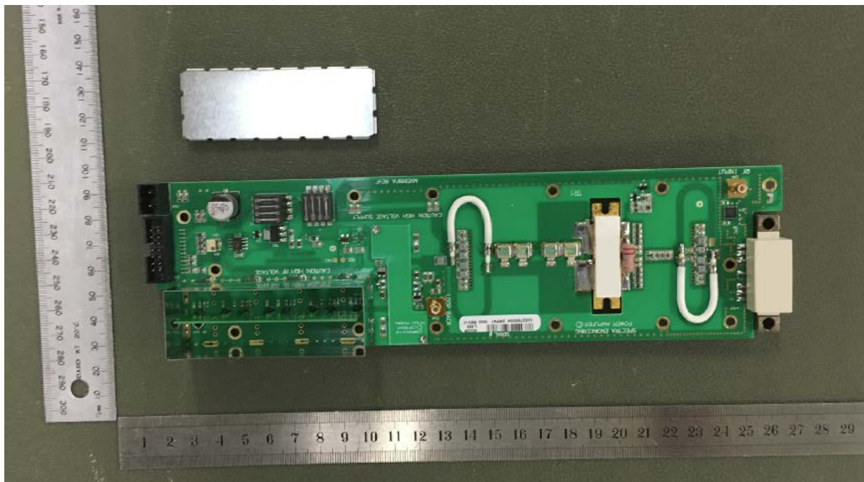
Figure 20. PA PCB Top View.
