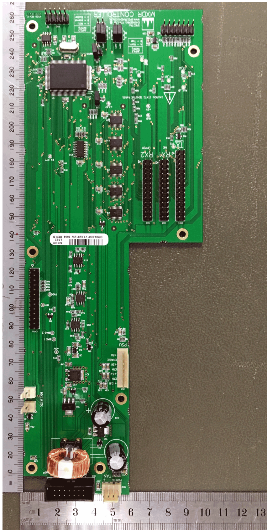
Figure 7. Controller PCB Top View.
