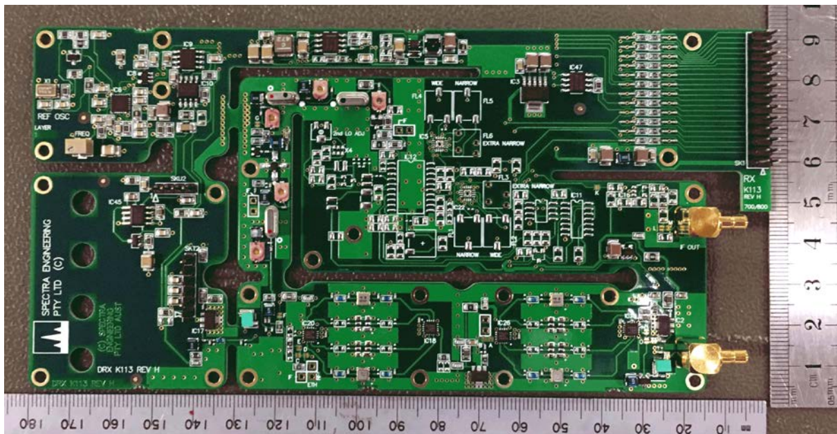
Figure 9. Receiver PCB Top View.
