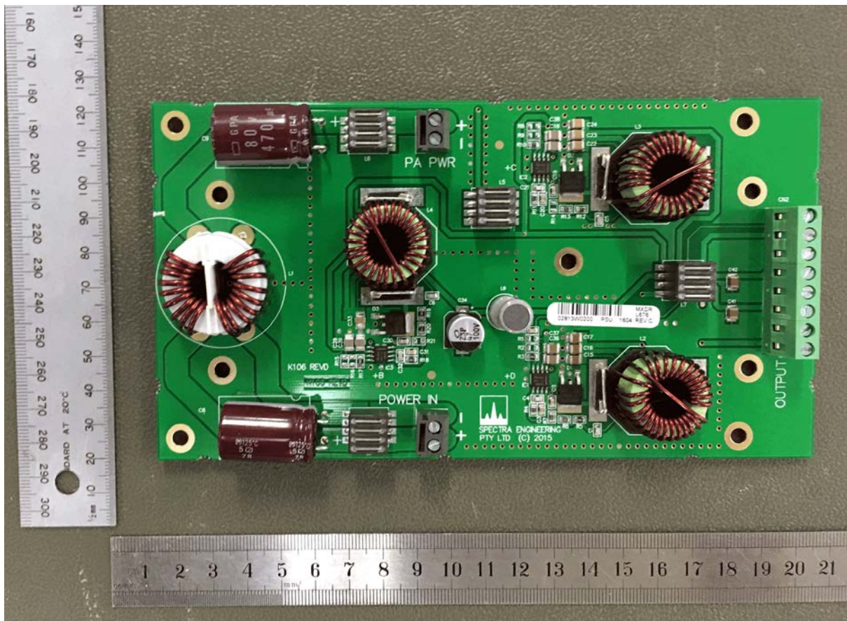
Figure 13. PSU PCB Top View.
