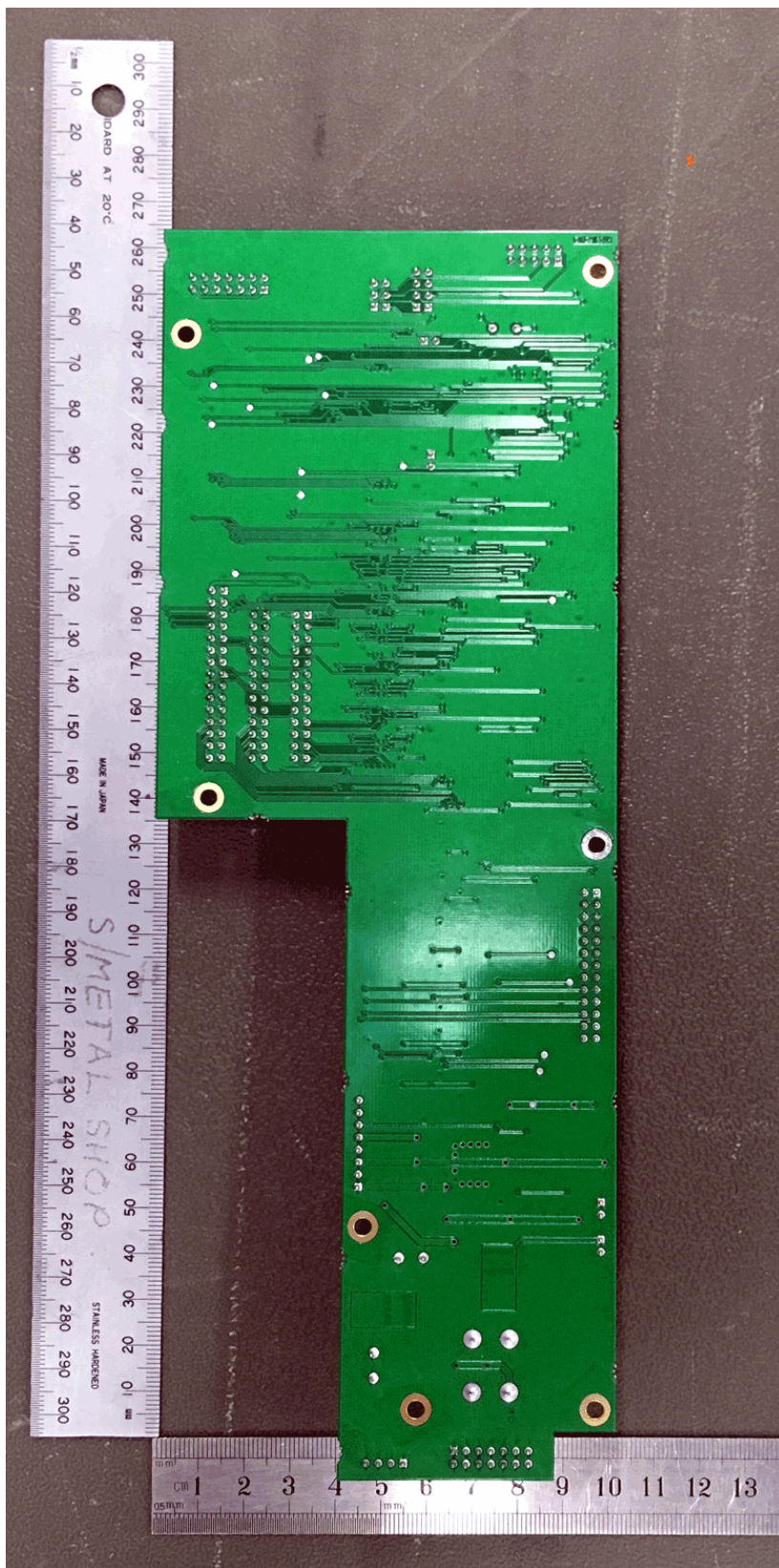
Figure 8. Controller PCB Bottom View.
