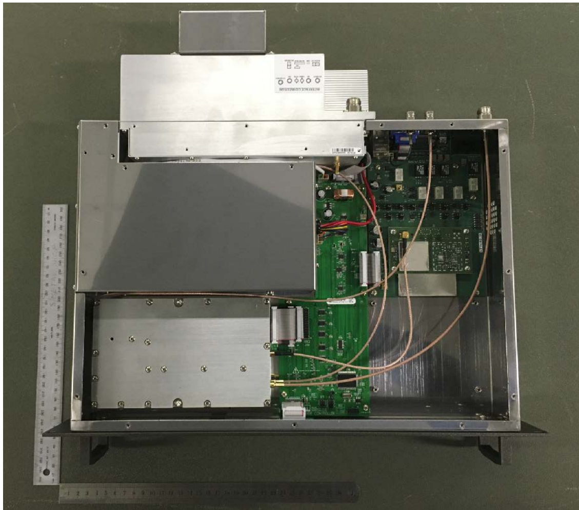
Figure 4. External Top View.
