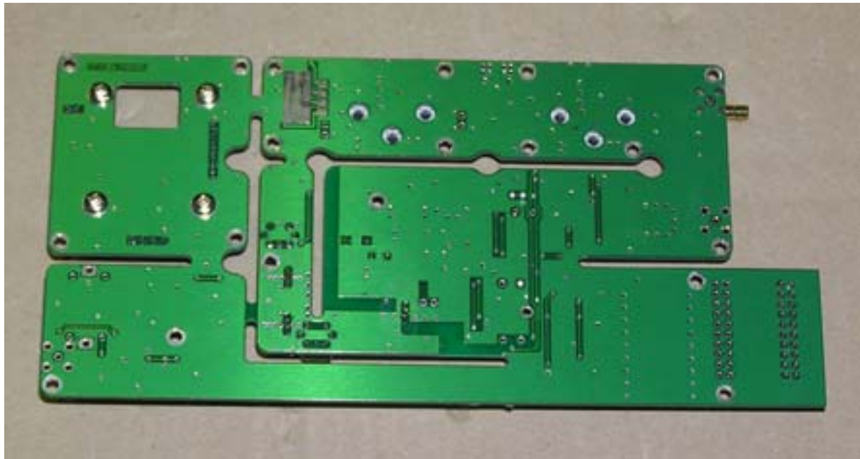
Receiver Bottom Photo
