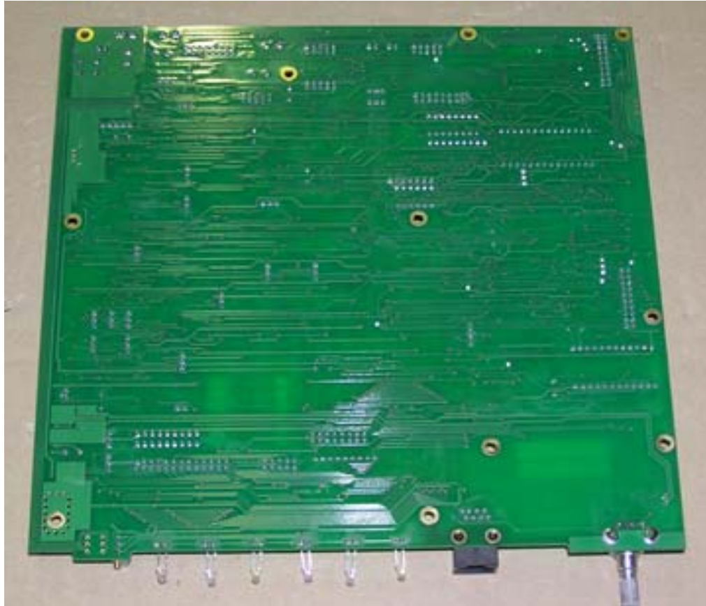
Mother Board Bottom Photo
