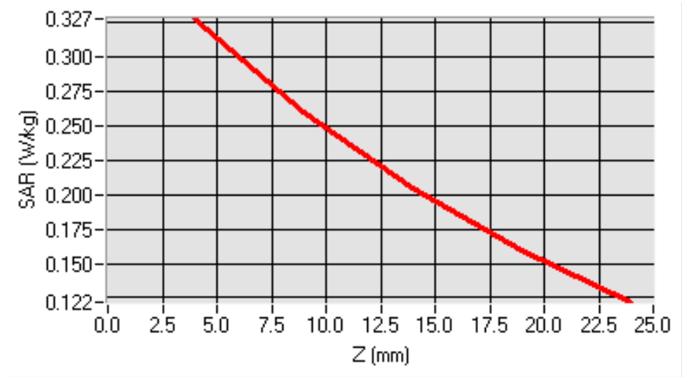
SAR, Z Axis Scan (X = -48, Y = -26)
