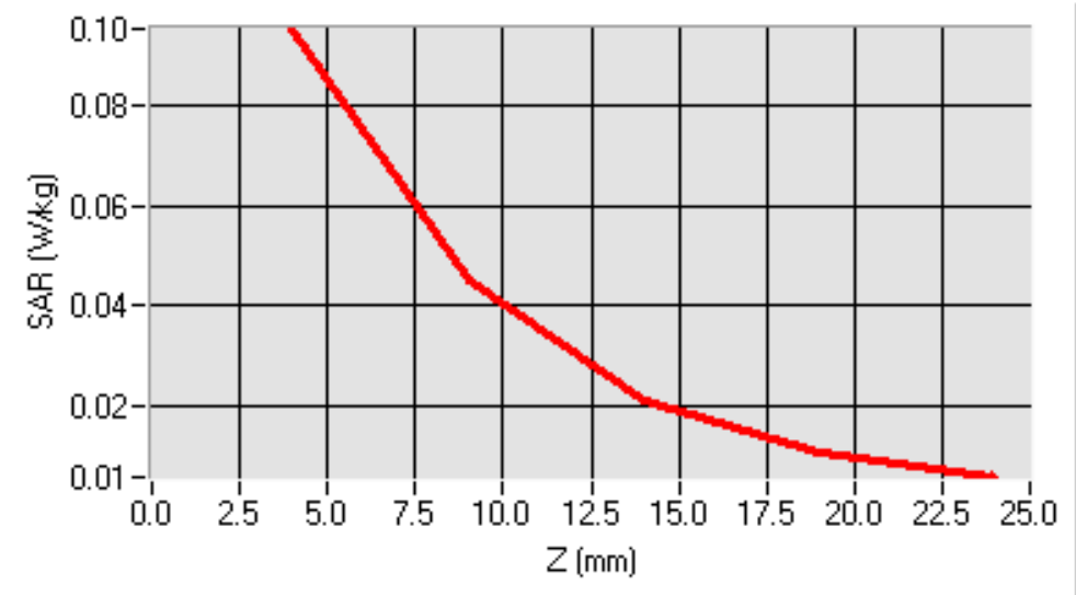
SAR, Z Axis Scan (X = 16, Y = -51)
