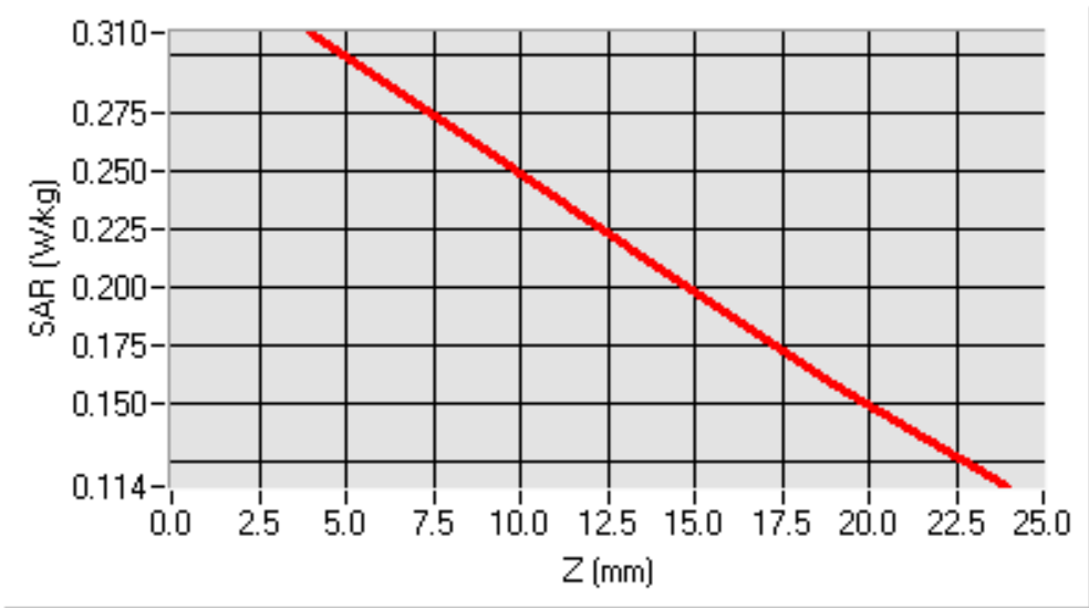
SAR, Z Axis Scan (X = -46, Y = -32)
