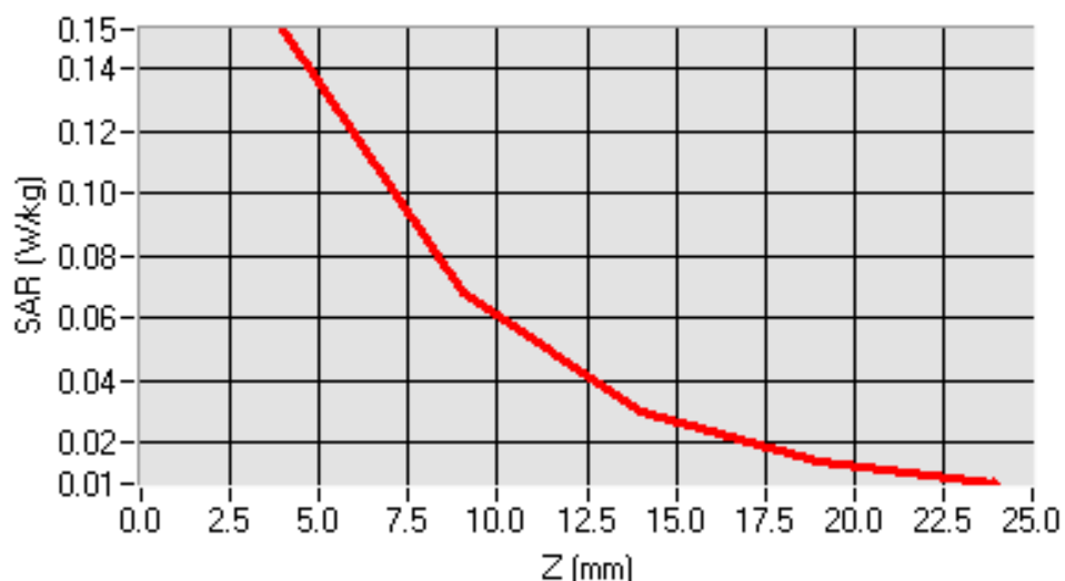
SAR, Z Axis Scan (X = -8, Y = -56)
