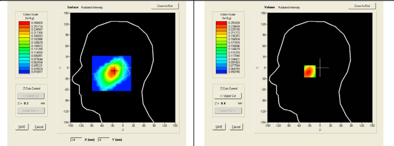
SAR, Z Axis Scan (X = -26, Y = -10)
