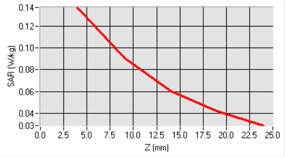
SAR, Z Axis Scan (X = -57, Y = -39)
