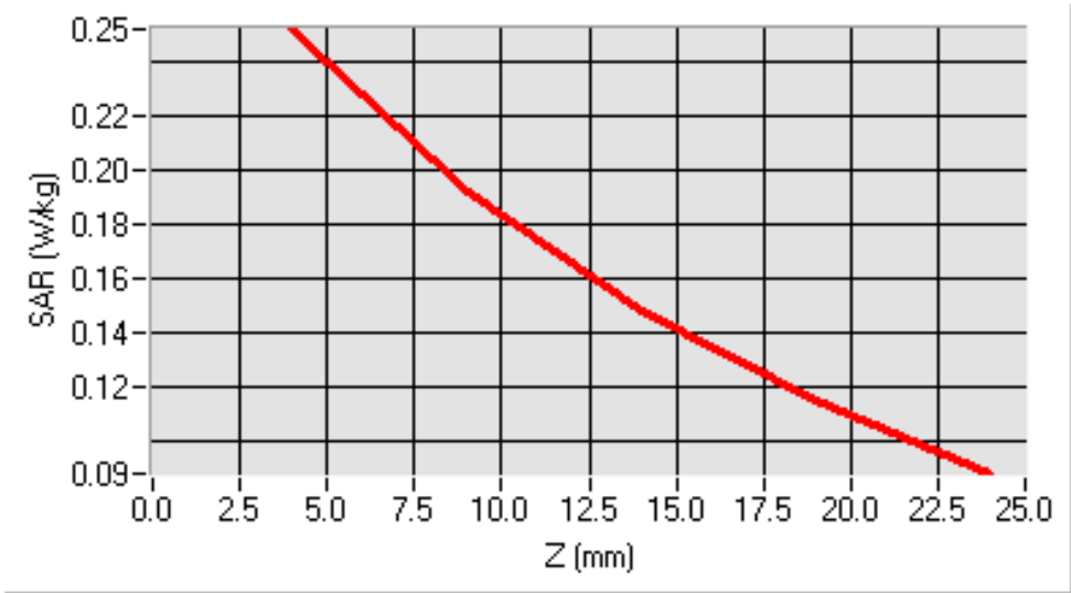
SAR, Z Axis Scan (X = -26, Y = -10)
