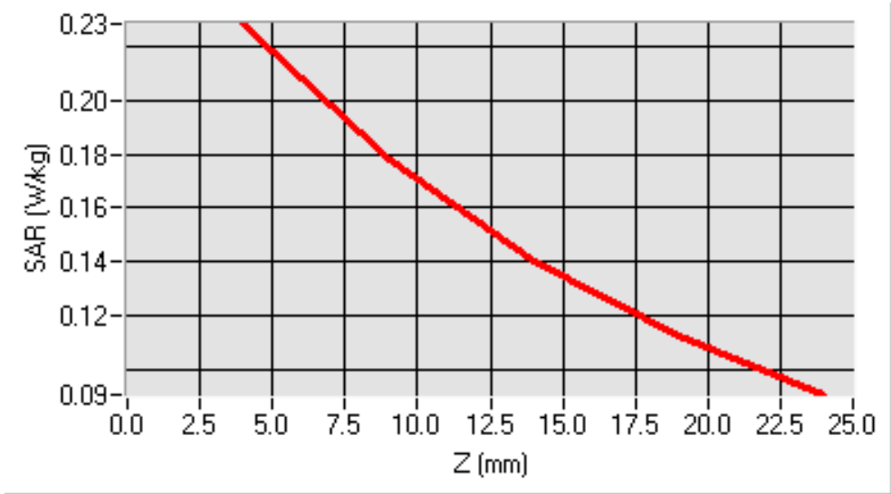
SAR, Z Axis Scan (X = -33, Y = -17)
