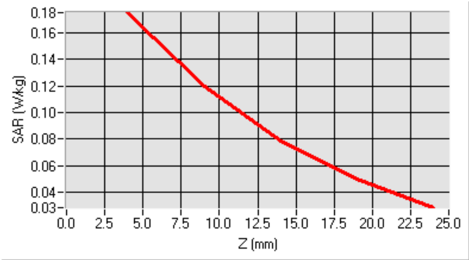
SAR, Z Axis Scan (X = -57, Y = -44)
