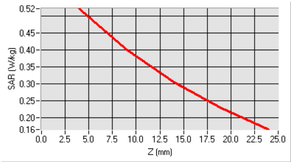
SAR, Z Axis Scan (X = 1, Y = -64)
