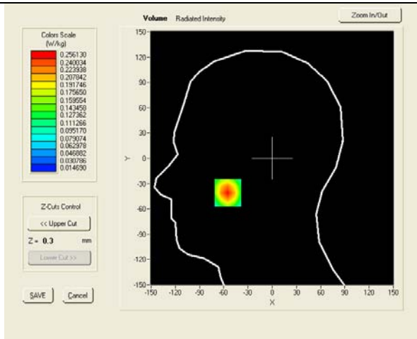
SAR, Z Axis Scan (X = -55, Y = -41)
