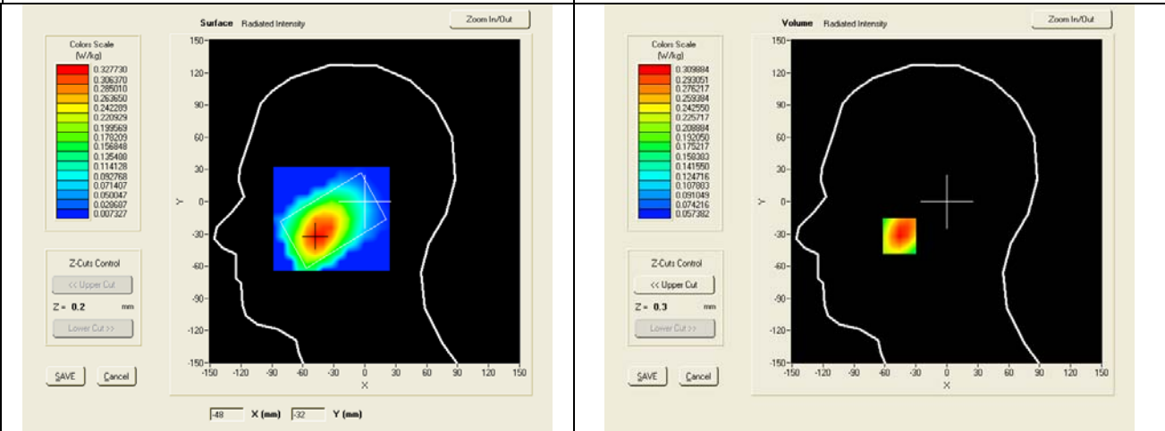
SAR, Z Axis Scan (X = -46, Y = -32)
