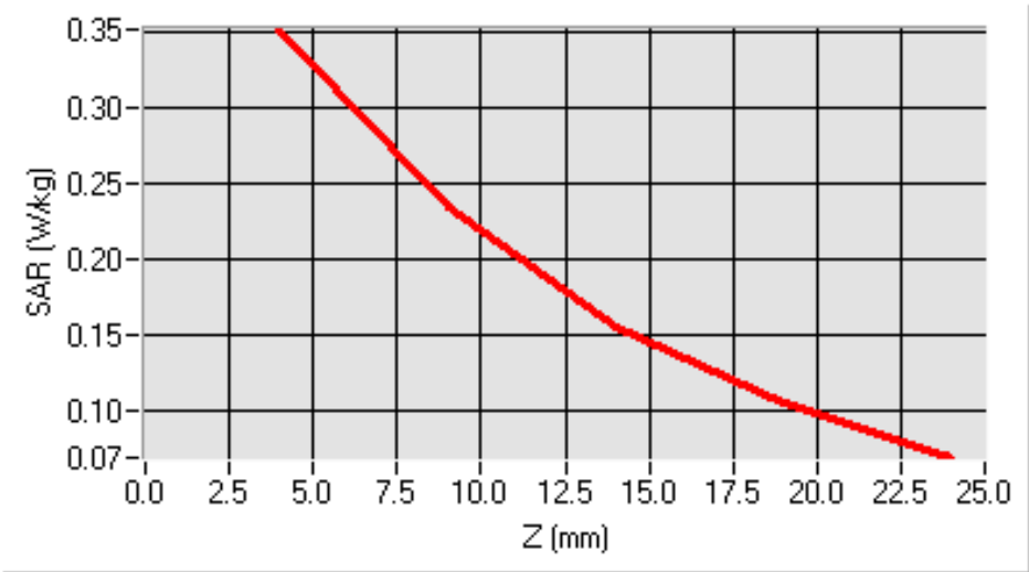
SAR, Z Axis Scan (X = -55, Y = -41)
