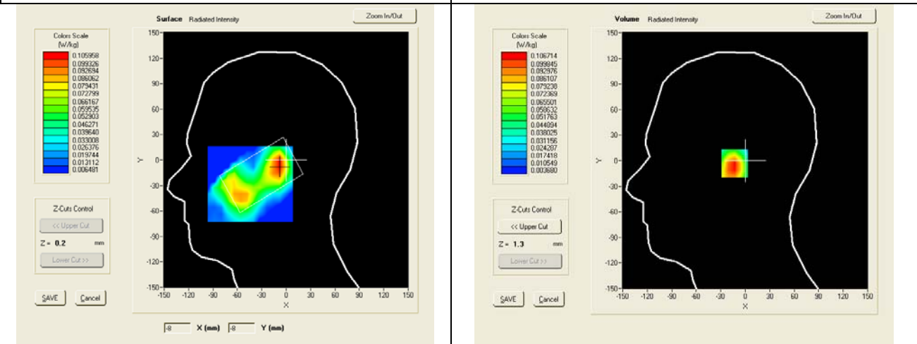
SAR, Z Axis Scan (X = -9, Y = -3)
