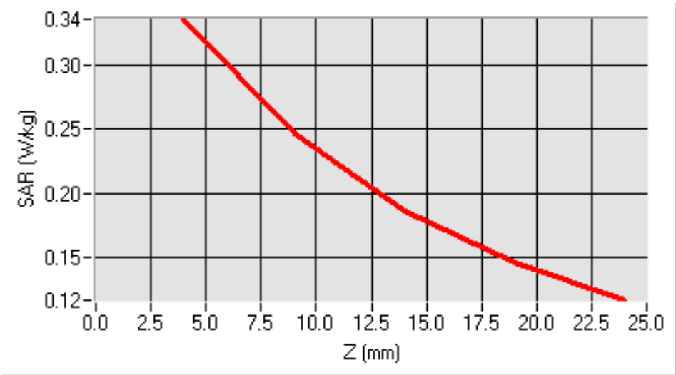
SAR, Z Axis Scan (X = -39, Y = -23)
