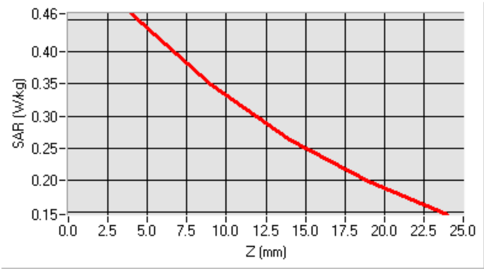
SAR, Z Axis Scan (X = -53, Y = -30)
