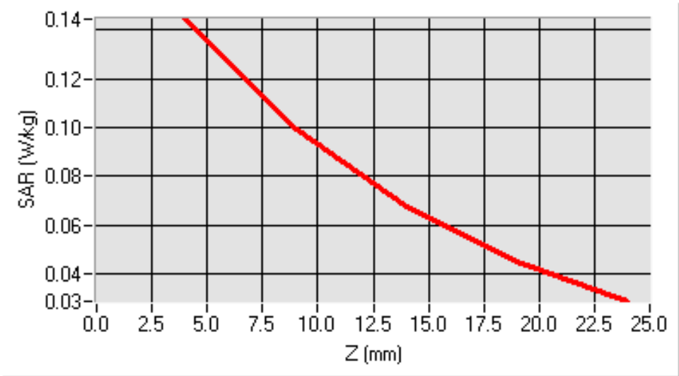
SAR, Z Axis Scan (X = -24, Y = 2)
