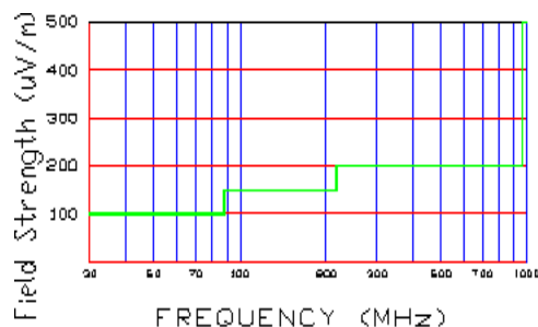
Figure 13. Spurious Radiated Limits at 3 meters © 1999 PCTEST Lab FCC ID: OKHCSW-244SC (2.410 – 2.470 GHz) C.T.I. CO., LTD. Wireless Camera Transmitter
