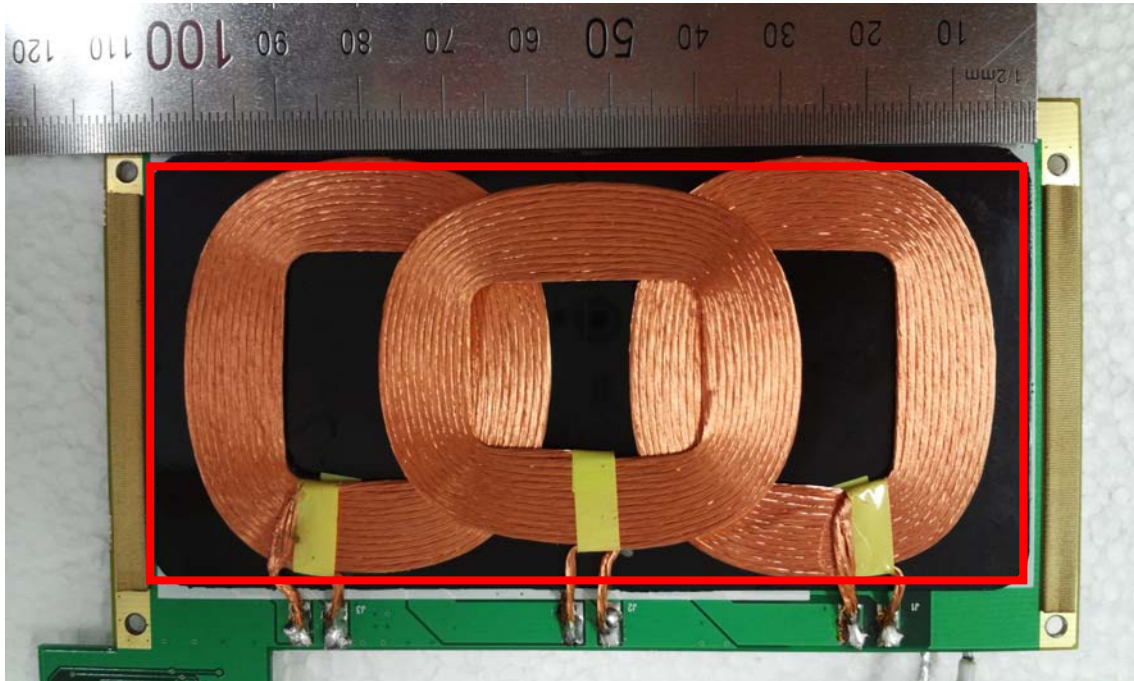
Internal View
