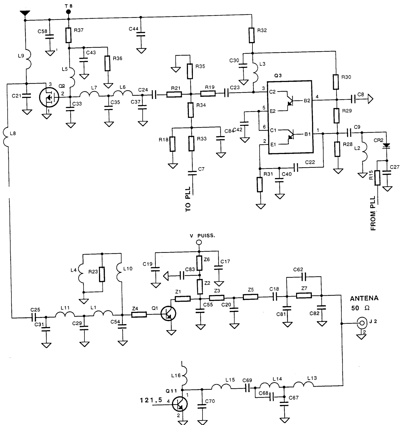
KANNAD 406 "WH"-97 UHF-VHF SCHEMATIC DIAGRAM I264 PCB
