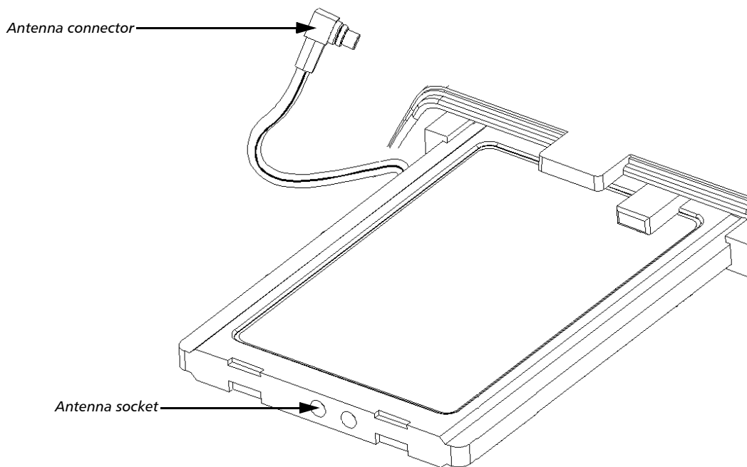
Figure 1-1: Connecting the Antenna to the PC Card
