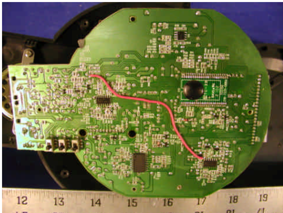
Base – Solder
