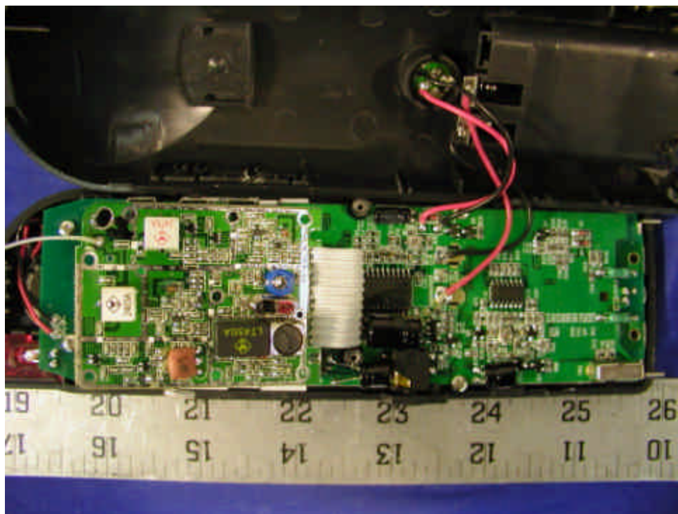
Handset – Solder
