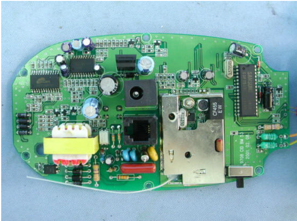
Base Main PCB comp side
