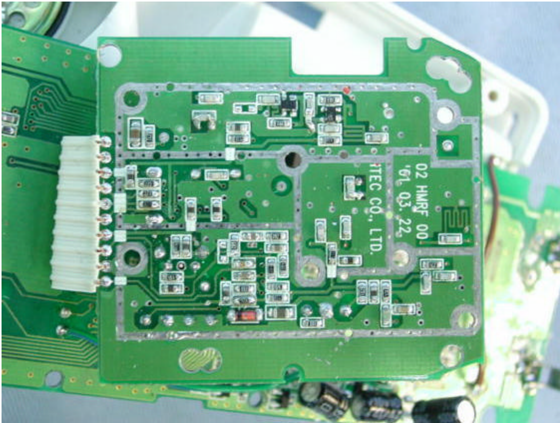
Handset Oscillator PCB solder side
