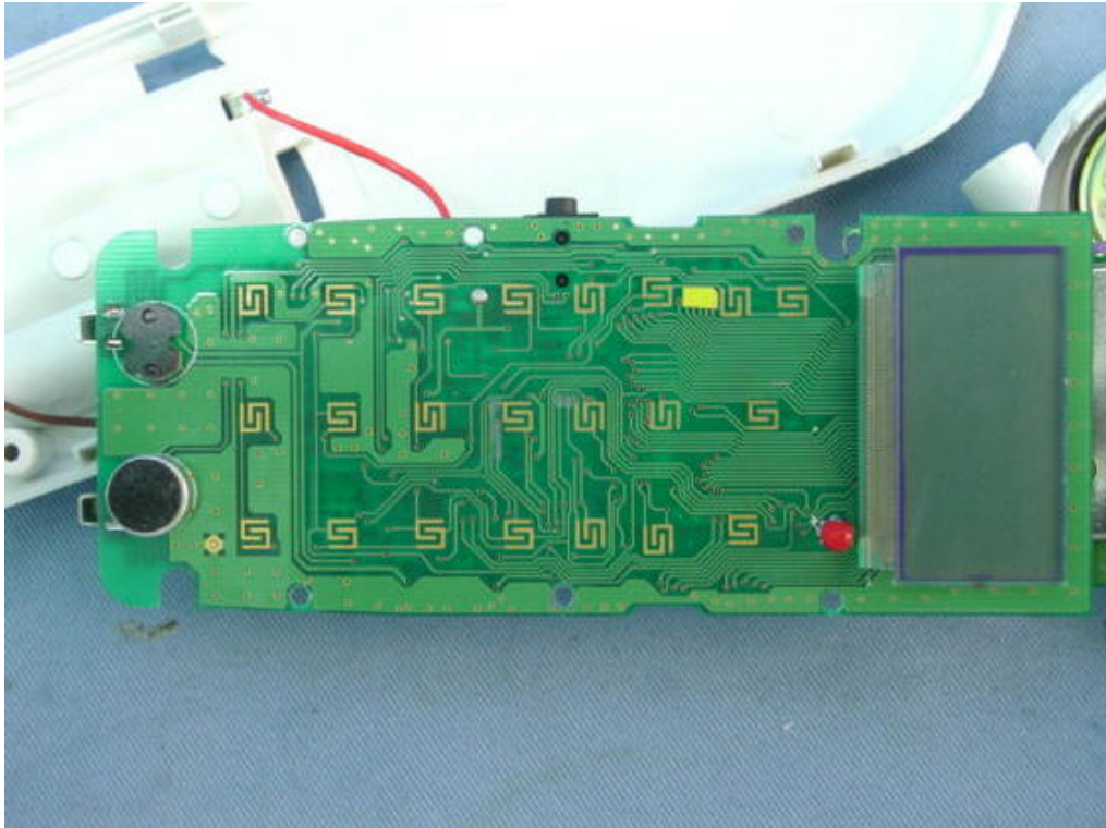
Handset Main PCB display side
