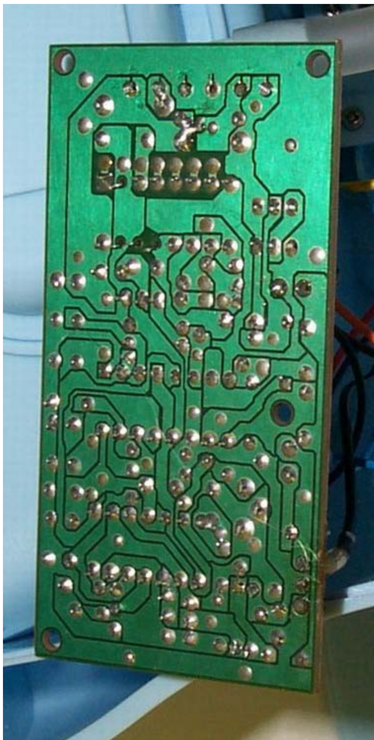
7.5 PCB1 Foil Side View
