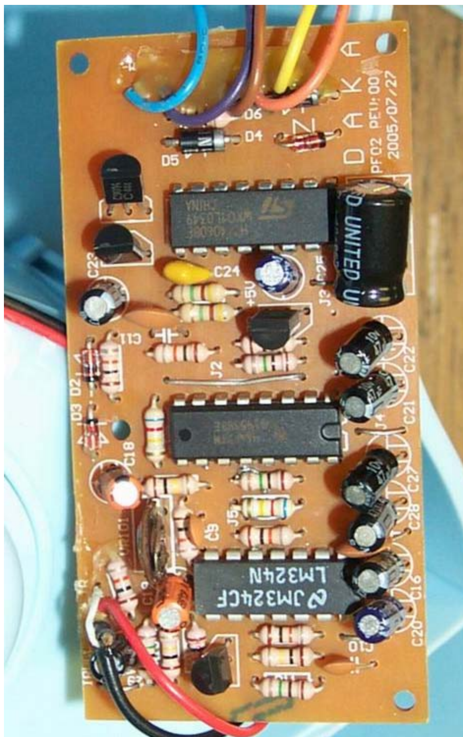
7.4 PCB1 Component Side View
