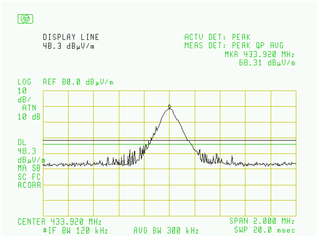
Figure 6.1 Occupied Bandwidth
