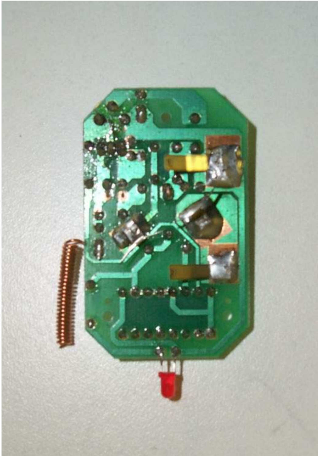
7.5 PCB Foil Side View
