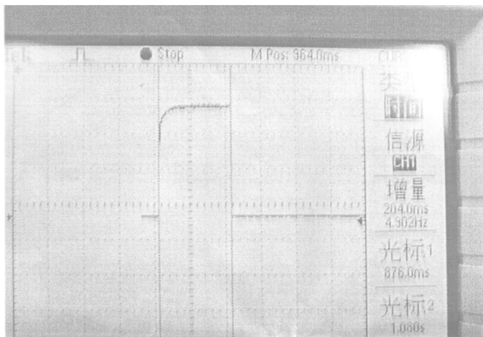
Figure 5.2 Duration of each transmission=204ms
