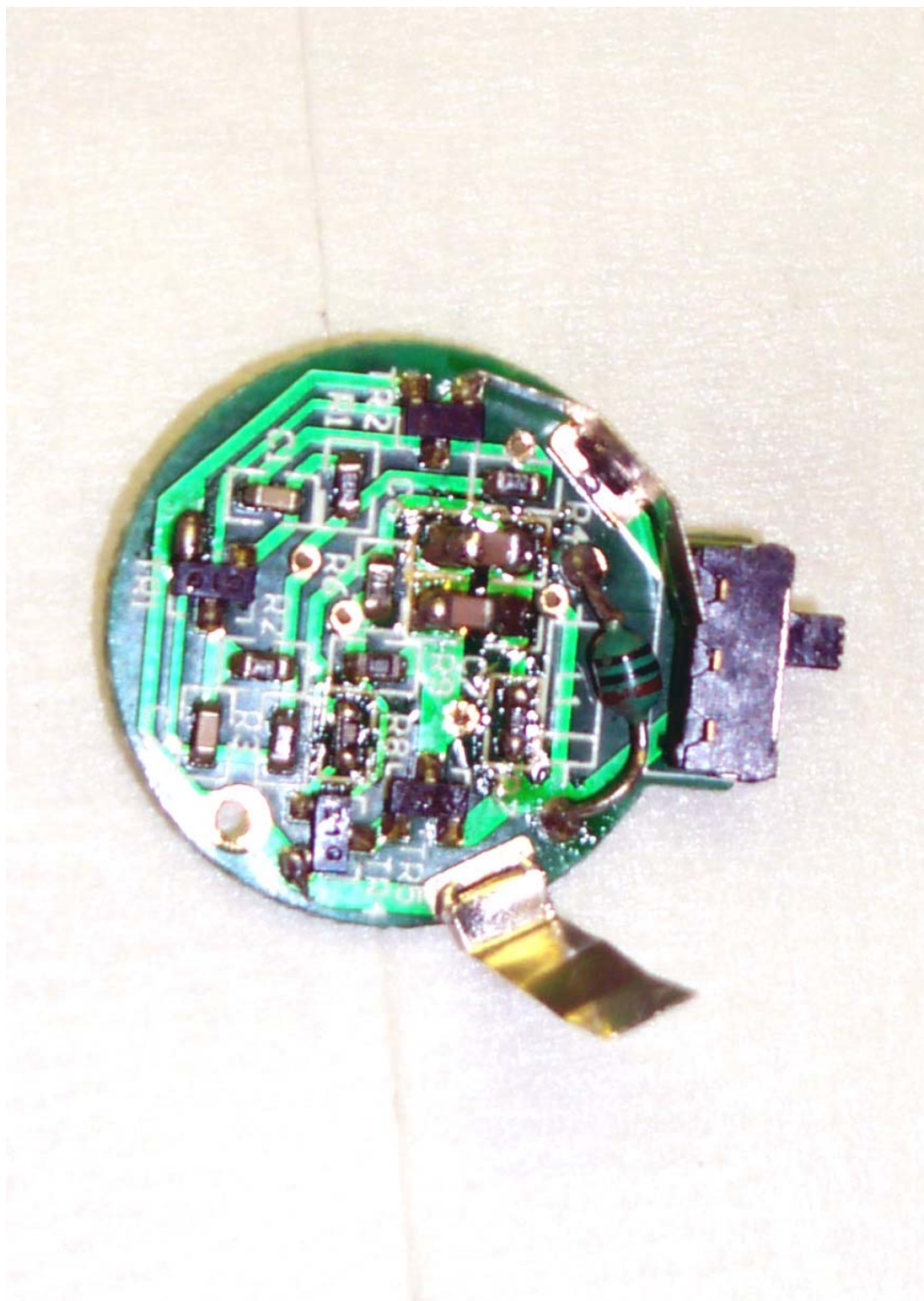
Component Side
