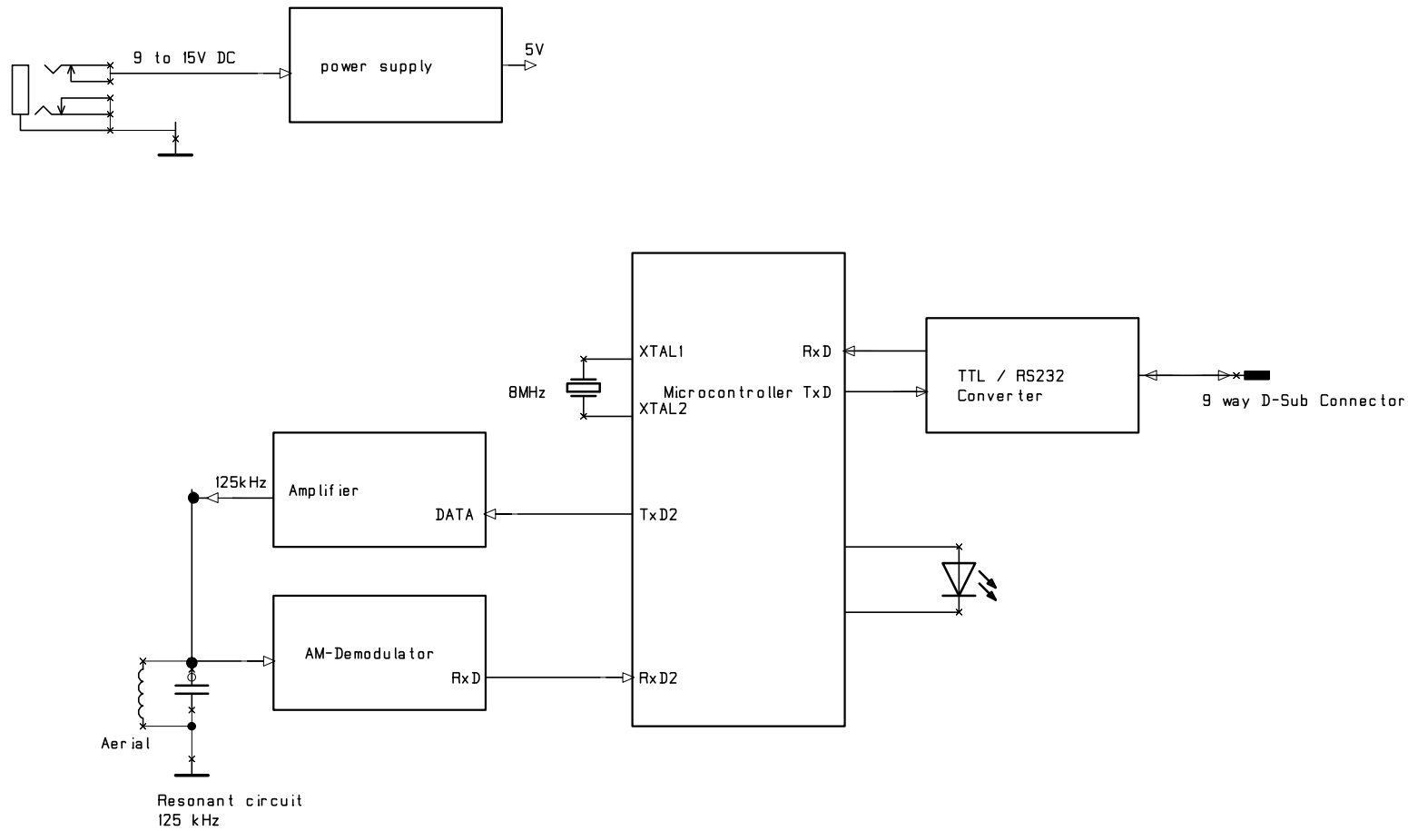
Block Diagram Pen-DTU
