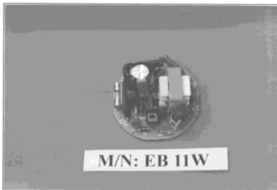
FIGURE 15 PCB BOARD (COMPONENT SIDE) (EB11W)
