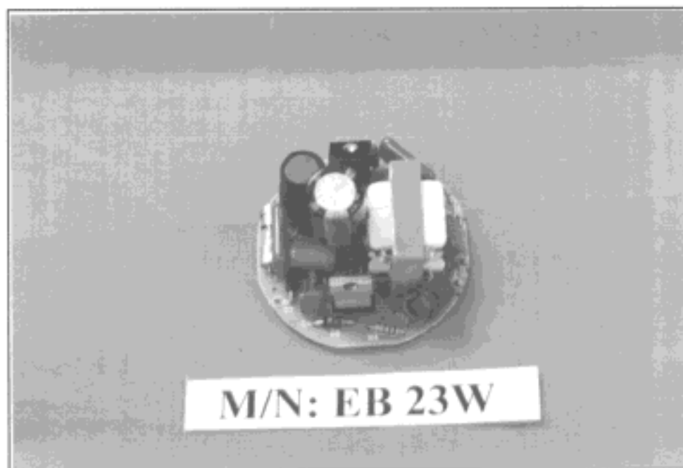
FIGURE 35 PCB BOARD (COMPONENT SIDE) (EB23W)
