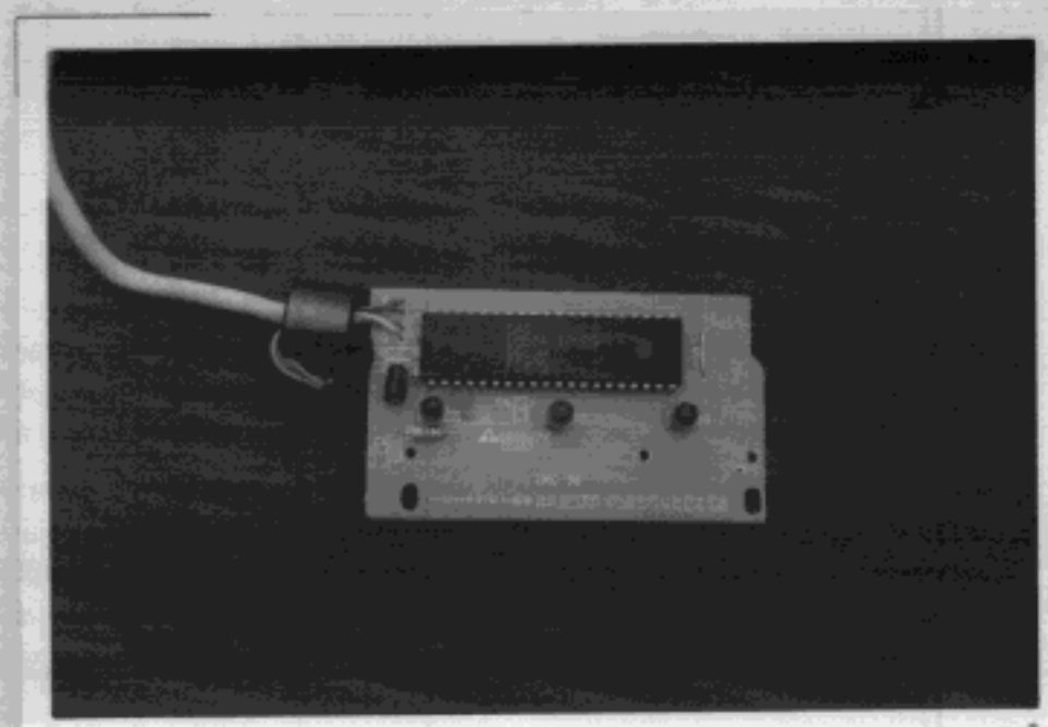
Figure 4 PCB Board, Component Side
