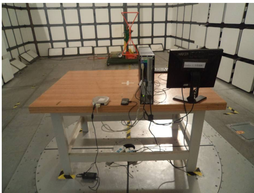
Radiated Emissions – Rear View (downloading mode)
