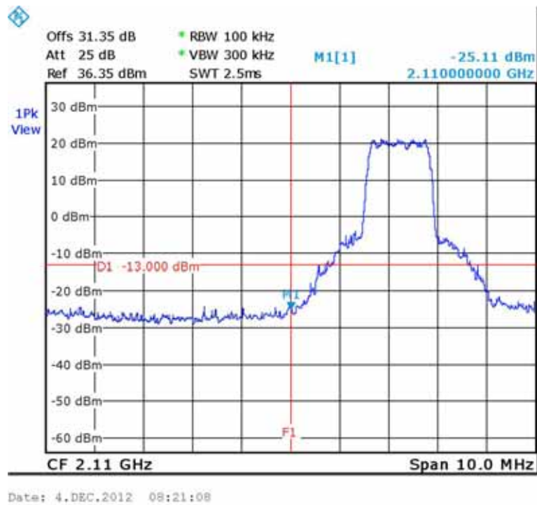
Figure 344.— CDMA 2112.20 MHz
