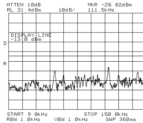
Figure 293.— 2153.80 MHz CDMA
