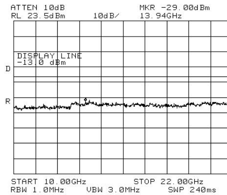
Figure 357 Intermodulation
