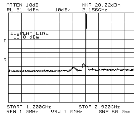
Figure 297.— 2153.80 MHz CDMA
