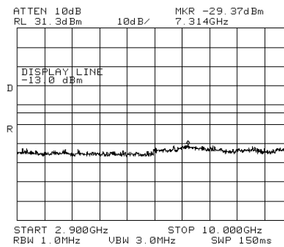
Figure 82.— 881.00 MHz
