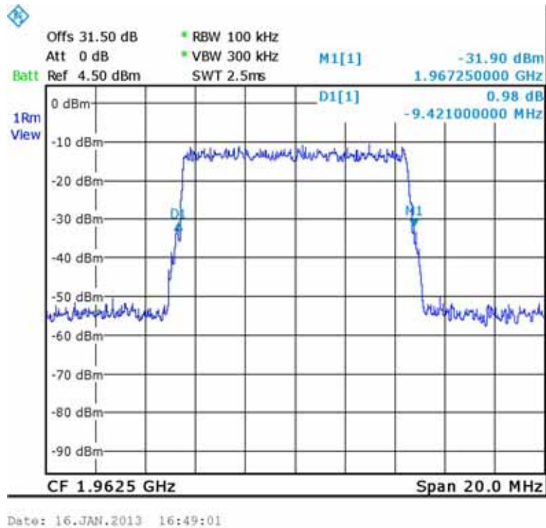
Figure 147.— 16QAM Input 1962.50 MHz
