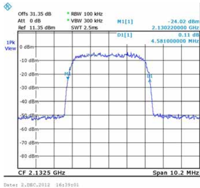
Figure 273.— W-CDMA (2132.5 MHz) IN
