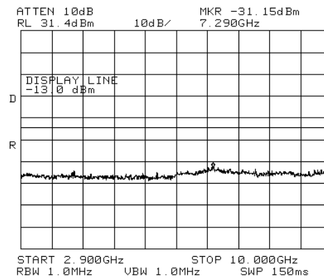
Figure 305.— 2115.00 MHz LTE
