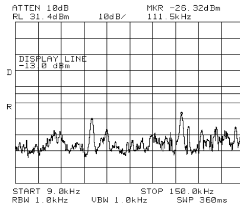
Figure 321.— 2112.50 MHz W-CDMA
