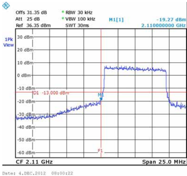
Figure 346.— LTE 2115.00 MHz
