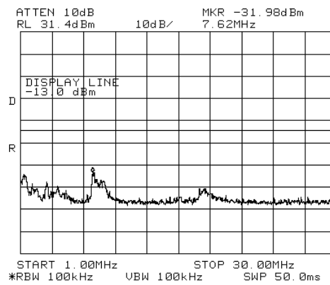
Figure 302.— 2115.00 MHz LTE
