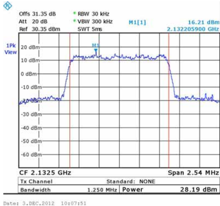
Figure 249.— CDMA (2132.5 MHz)
