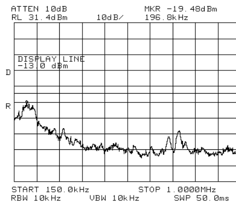
Figure 307.— 2132.50 MHz LTE
