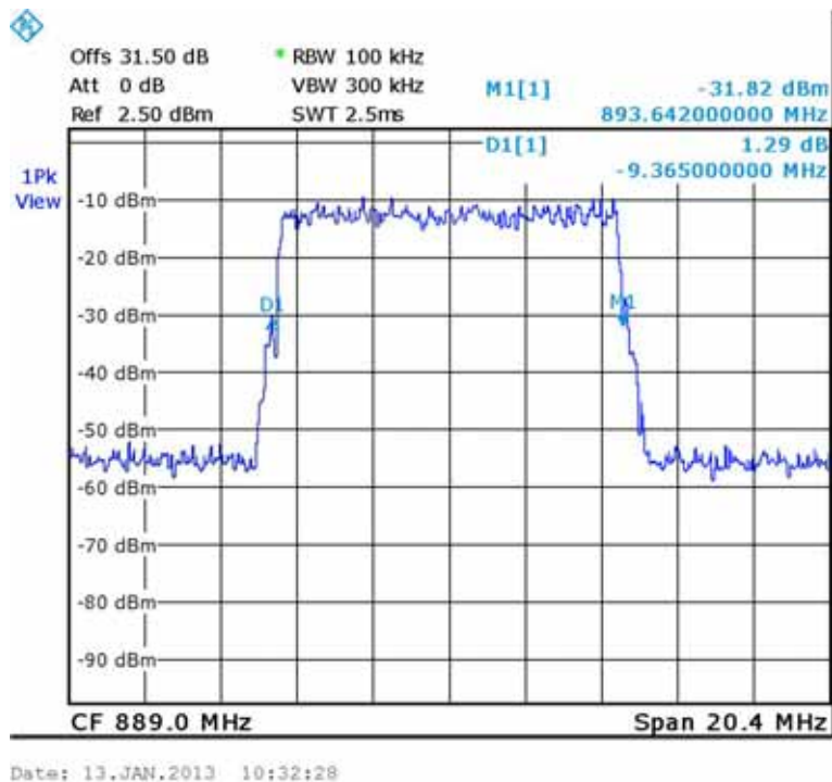
Figure 26.— 64QAM Input 889.00 MHz.
