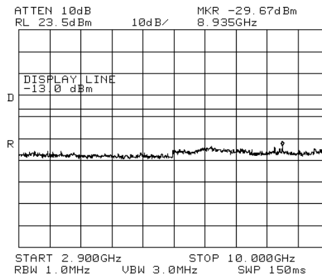
Figure 356 Intermodulation
