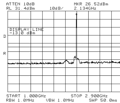
Figure 290.— 2132.50 MHz CDMA
