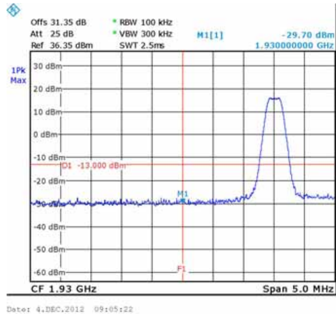
Figure 242.— 1931.20 MHz
