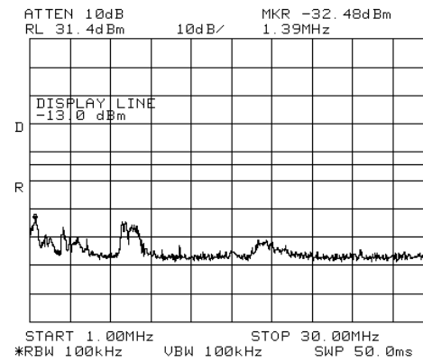
Figure 330.— 2132.50 MHz W-CDMA
