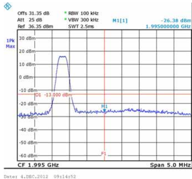
Figure 243.— 1993.80 MHz
