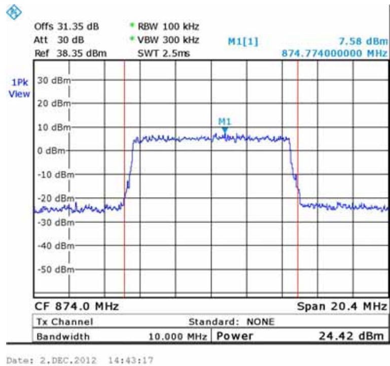
Figure 11.— 874.00 MHz
