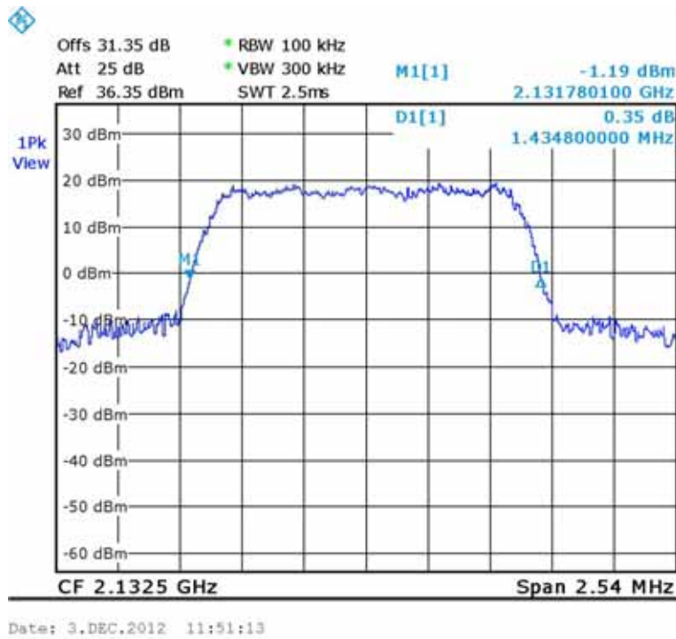
Figure 262.— CDMA (2132.5 MHz) OUT
