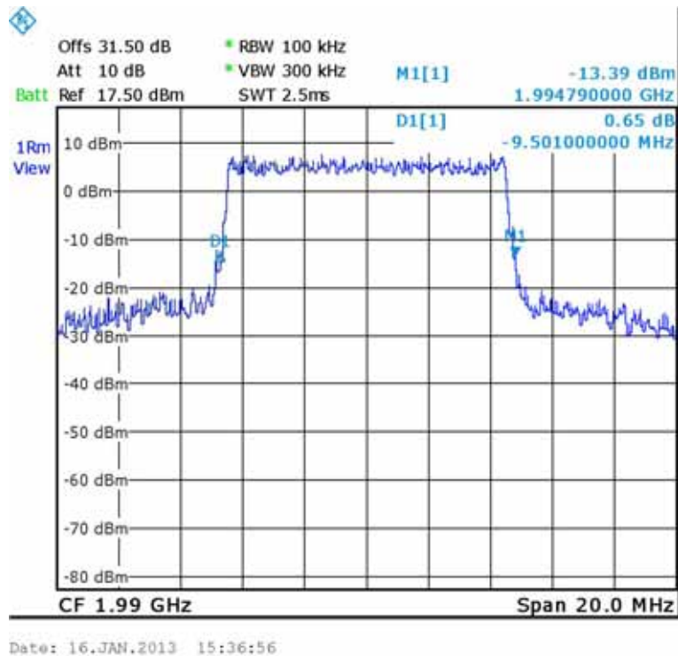
Figure 155.— QPSK Input 1990.00 MHz
