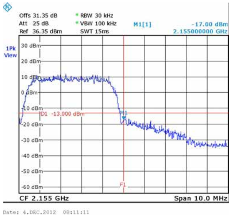
Figure 349.— W-CDMA 2152.50 MHz
