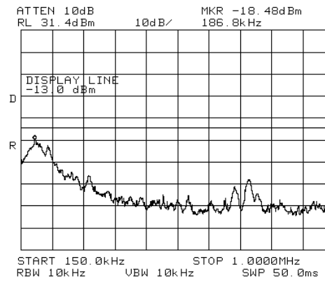
Figure 329.— 2132.50 MHz W-CDMA
