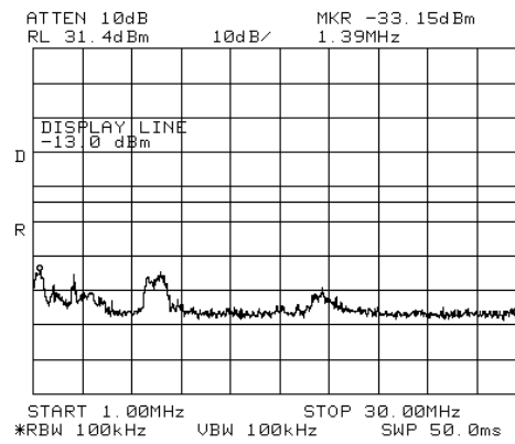
Figure 337.— 2152.50 MHz W-CDMA
