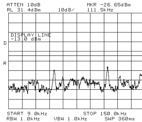
Figure 335.— 2152.50 MHz W-CDMA
