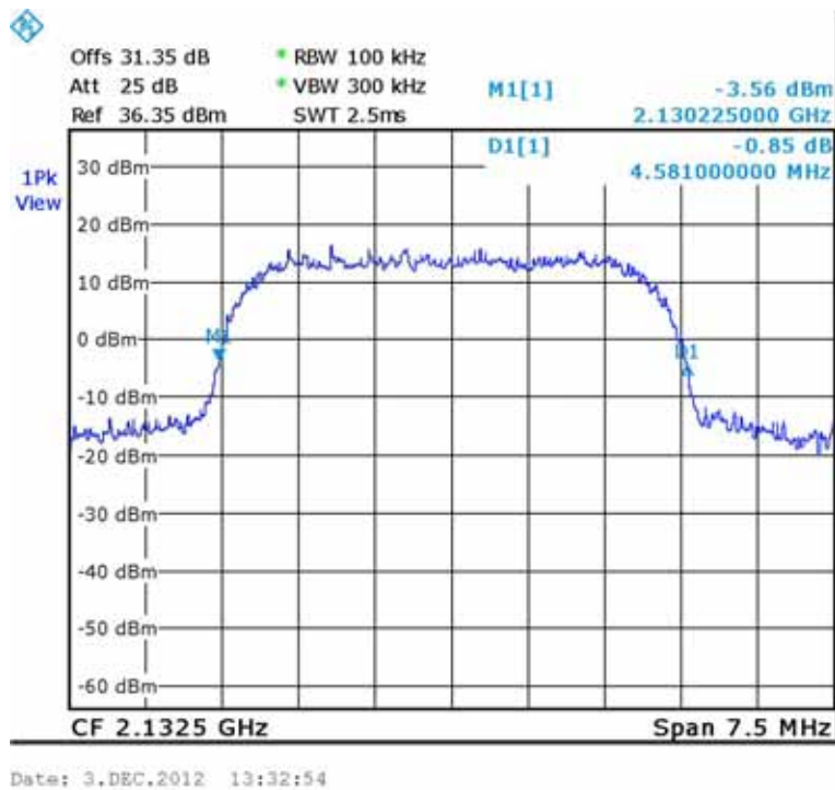
Figure 274.— W-CDMA (2132.5 MHz) OUT
