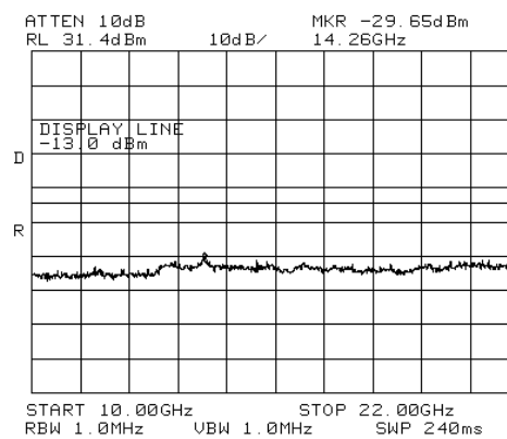
Figure 299.— 2153.80 MHz CDMA
