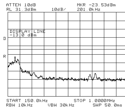
Figure 90.— 871.50 MHz
