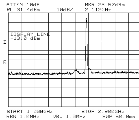
Figure 325.— 2112.50 MHz W-CDMA
