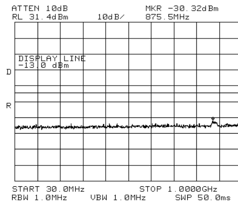
Figure 303.— 2115.00 MHz LTE
