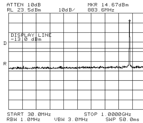
Figure 354 Intermodulation
