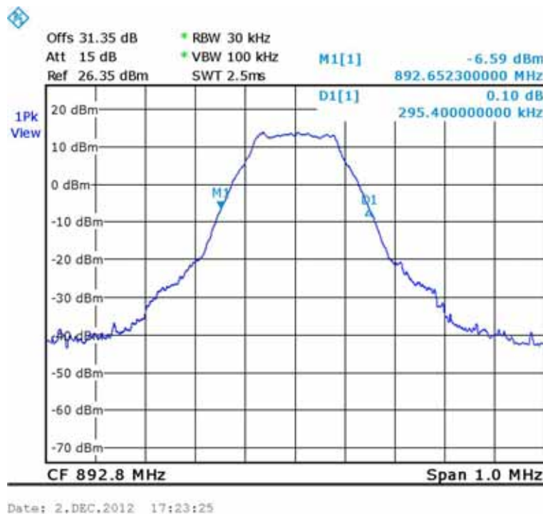
Figure 45.— Output 892.8 MHz.
