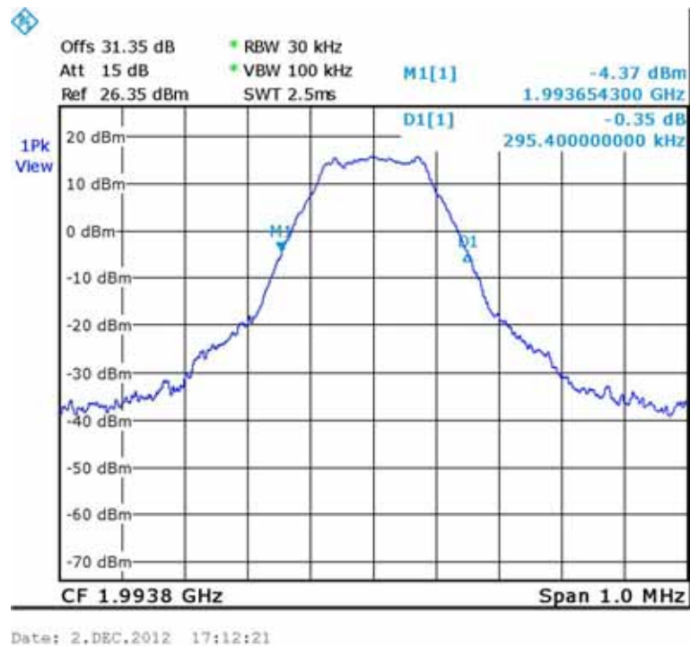
Figure 162.— Output 1993.80 MHz
