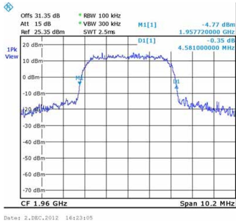
Figure 166.— Output 1960.00 MHz
