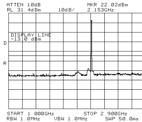
Figure 318.— 2151.00 MHz LTE
