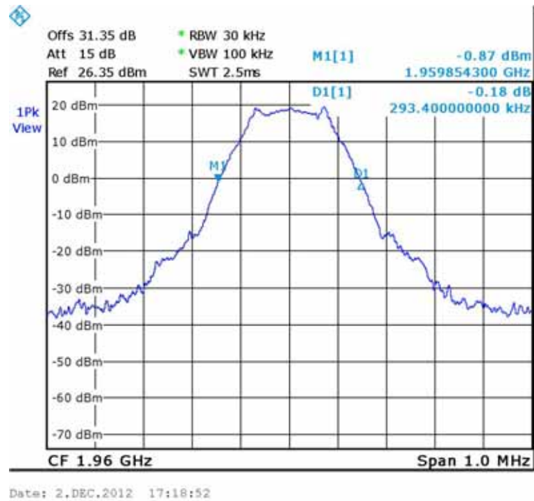
Figure 160.— Output 1960.00 MHz
