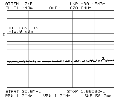
Figure 317.— 2151.00 MHz LTE
