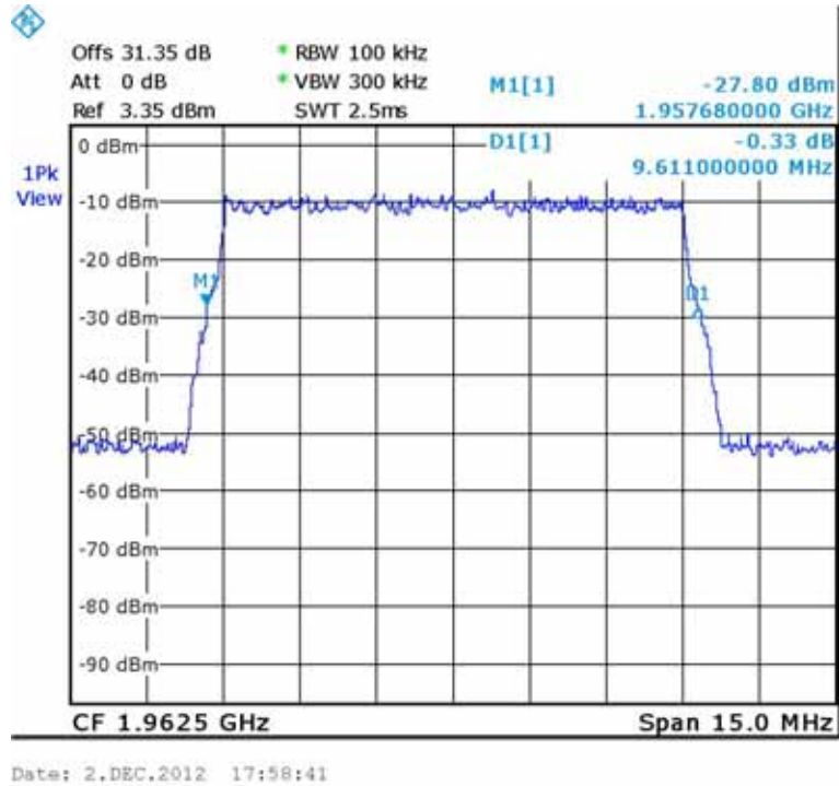
Figure 141.— 64QAM Input 1962.50 MHz
