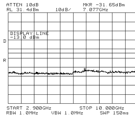
Figure 284.— 2112.20 MHz CDMA
