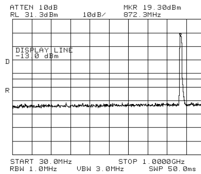
Figure 56.— 874.00 MHz
