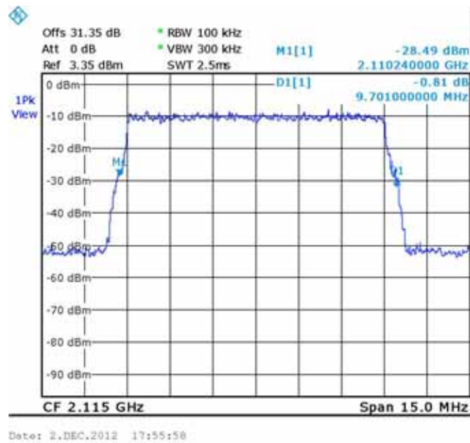
Figure 265.— LTE (2115.0 MHz) IN
