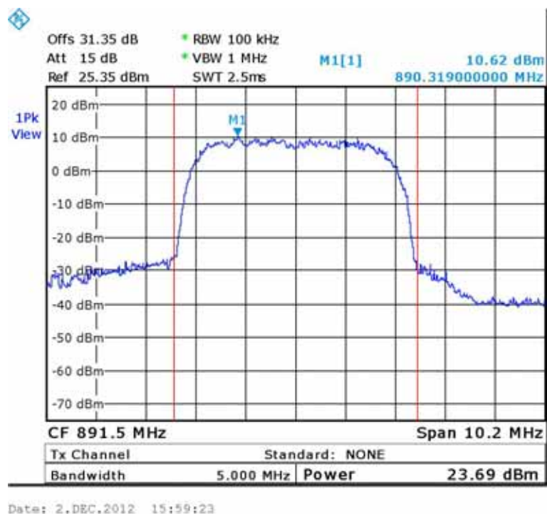
Figure 19.— 891.50 MHz
