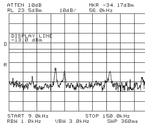
Figure 351 Intermodulation
