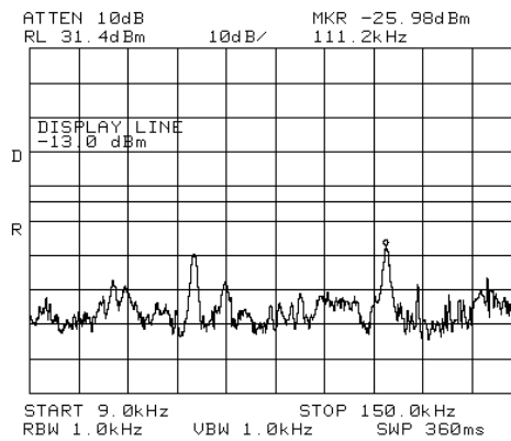
Figure 327.— 2112.50 MHz W-CDMA
