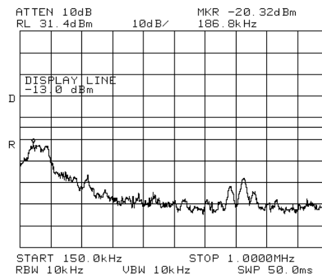
Figure 321.— 2112.50 MHz W-CDMA
