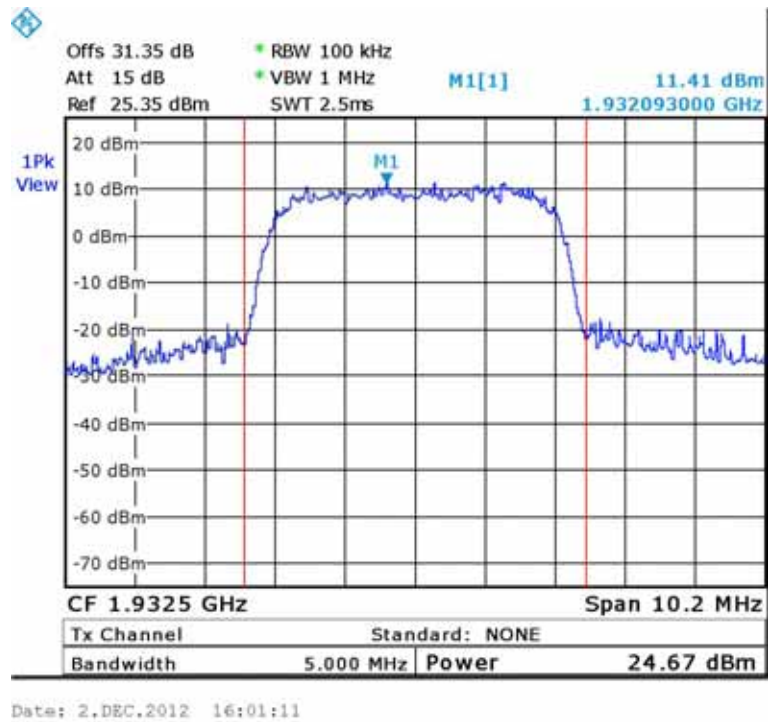
Figure 134.— 1932.50 MHz
