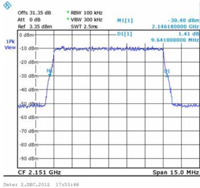
Figure 269.— LTE (2151.0 MHz) IN
