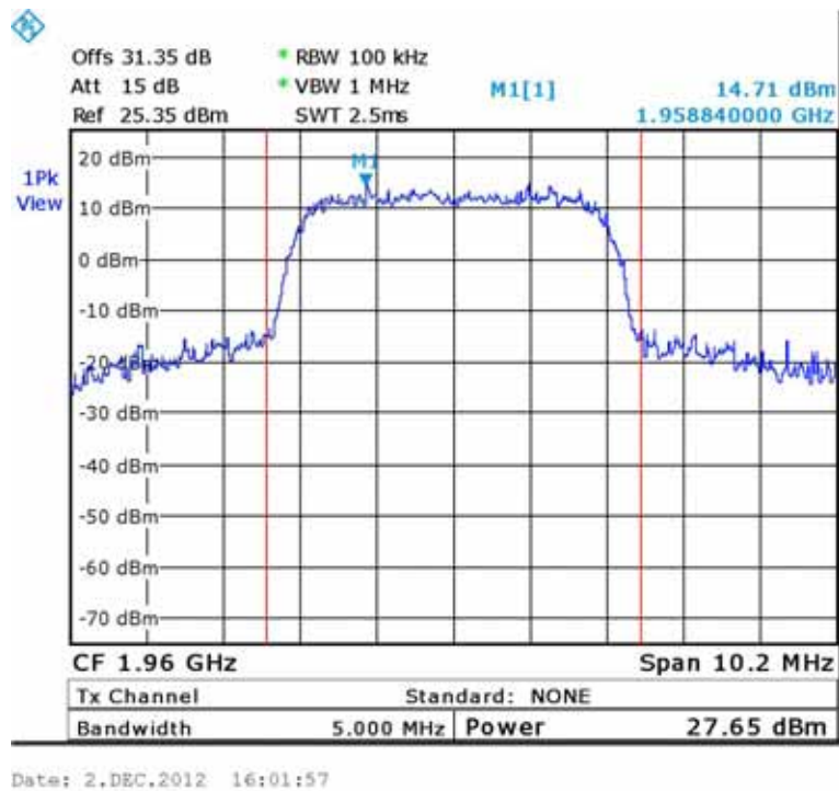
Figure 135.— 1960.00 MHz
