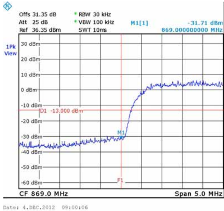
Figure 118.— 871.50 MHz
