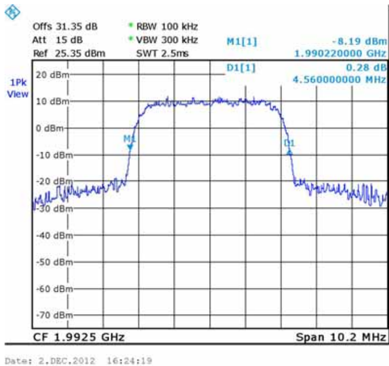
Figure 168.— Output 1992.50 MHz
