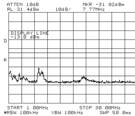
Figure 309.— 2132.50 MHz LTE
