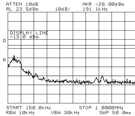
Figure 352 Intermodulation
