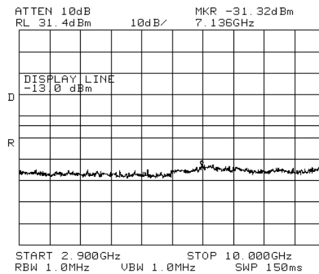
Figure 339.— 2152.50 MHz W-CDMA
