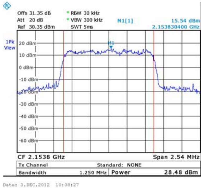
Figure 250.— CDMA (2153.8 MHz)
