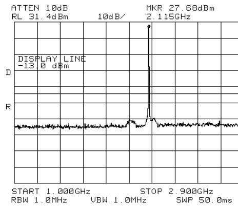
Figure 283.— 2112.20 MHz CDMA
