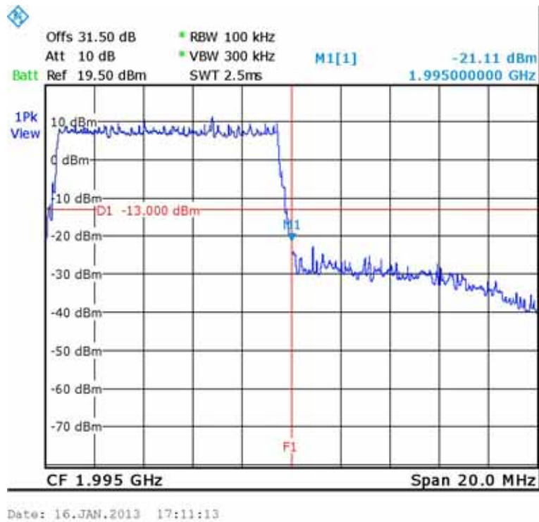
Figure 241.— QPSK 1990.00 MHz
