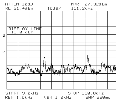
Figure 286.— 2132.50 MHz CDMA
