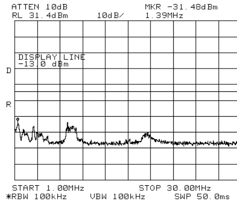
Figure 281.— 2112.20 MHz CDMA
