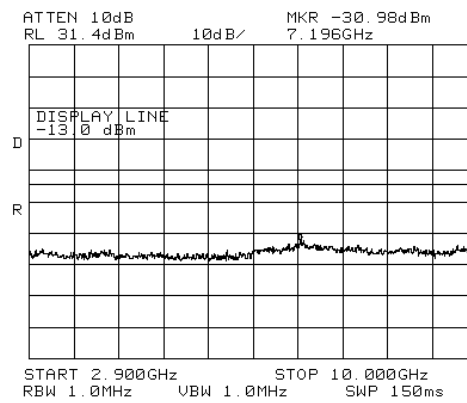
Figure 298.— 2153.80 MHz CDMA
