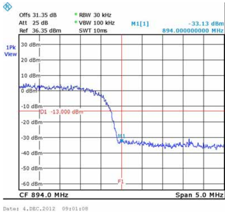
Figure 119.— 891.50 MHz
