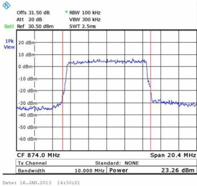
Figure 5.— 874.00 MHz
