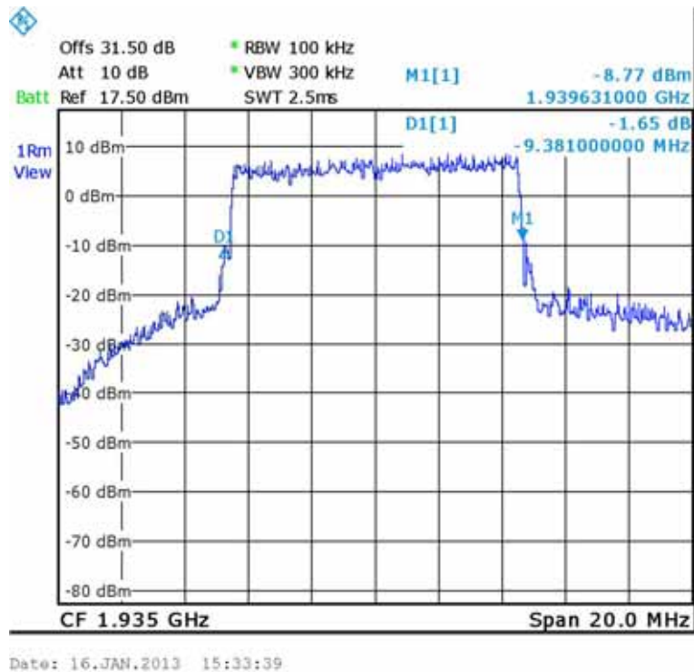
Figure 151.— QPSK Input 1935.00 MHz
