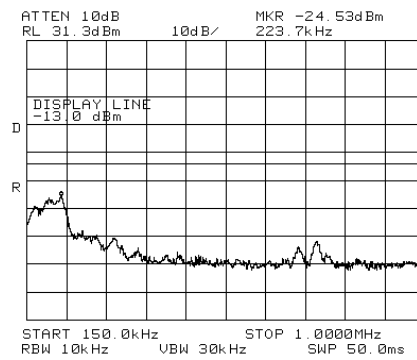
Figure 72.— 870.20 MHz
