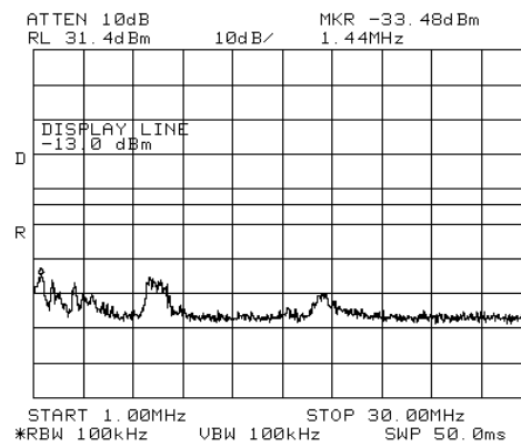
Figure 295.— 2153.80 MHz CDMA
