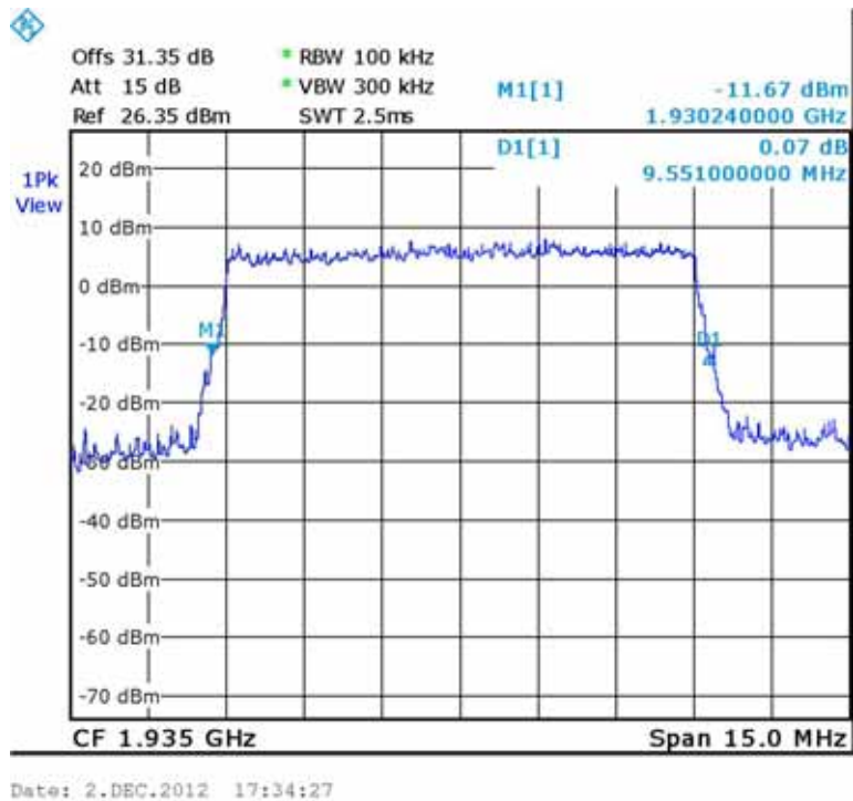
Figure 140.— 64QAM Output 1935.00 MHz
