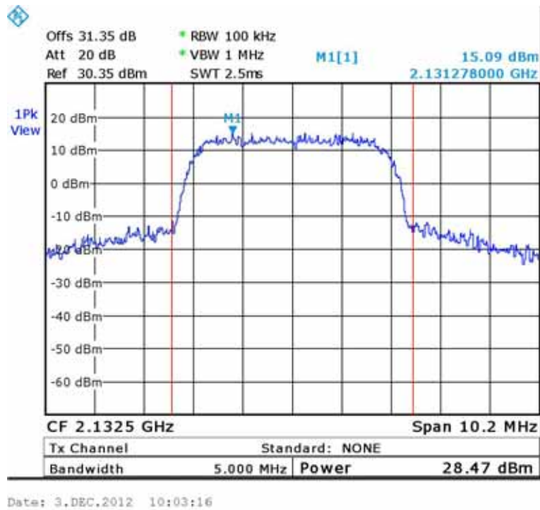
Figure 255.— W-CDMA (2132.5 MHz)
