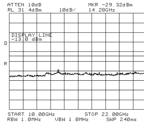
Figure 313.— 2132.50 MHz LTE
