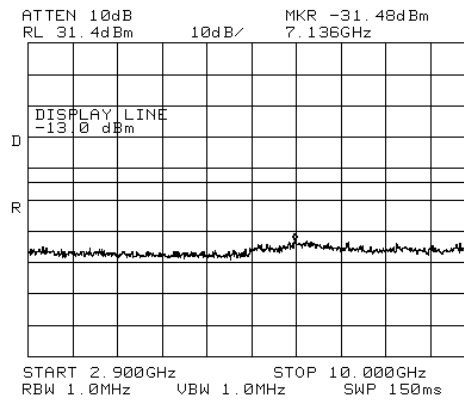
Figure 312.— 2132.50 MHz LTE
