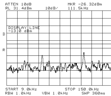
Figure 279.— 2112.20 MHz CDMA
