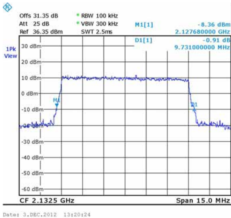
Figure 267.— LTE (2132.5 MHz) IN
