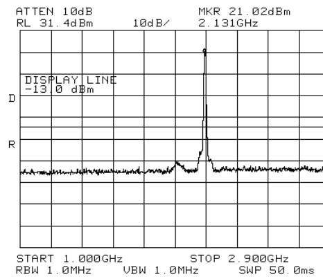
Figure 331.— 2132.50 MHz W-CDMA
