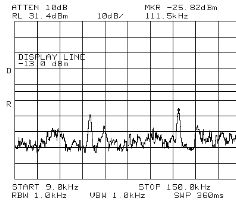
Figure 307.— 2132.50 MHz LTE
