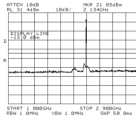
Figure 311.— 2132.50 MHz LTE
