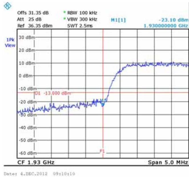
Figure 244.— 1932.50 MHz
