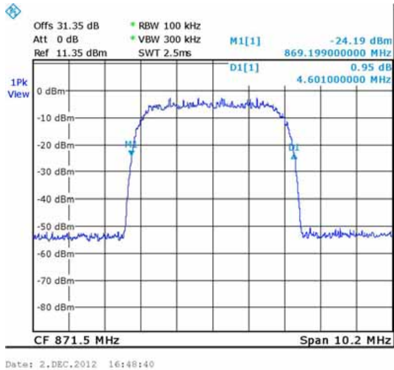
Figure 46.— Input 871.50
