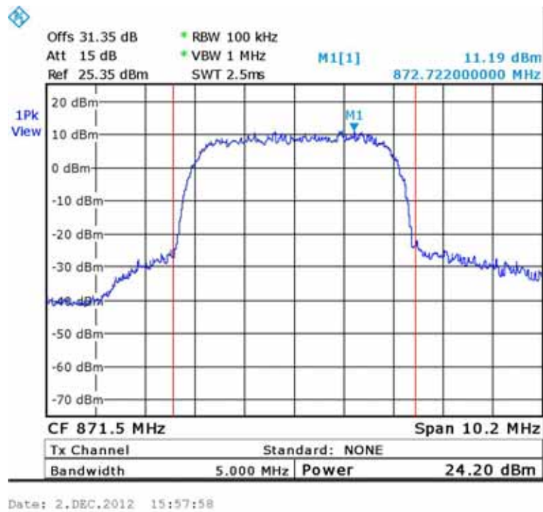
Figure 17.— 871.50 MHz
