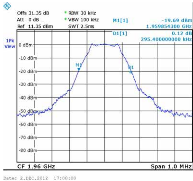
Figure 159.— Input 1960.00 MHz
