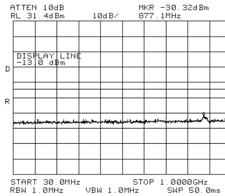
Figure 310.— 2132.50 MHz LTE
