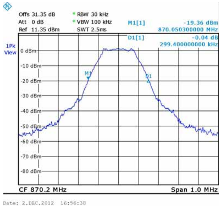
Figure 40.— Input 870.20
