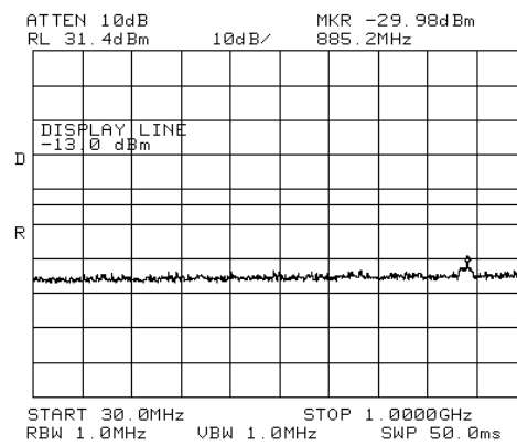
Figure 323.— 2112.50 MHz W-CDMA
