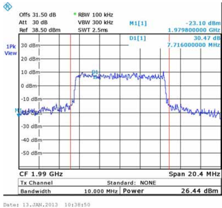
Figure 124.— 64QAM 1990.00 MHz
