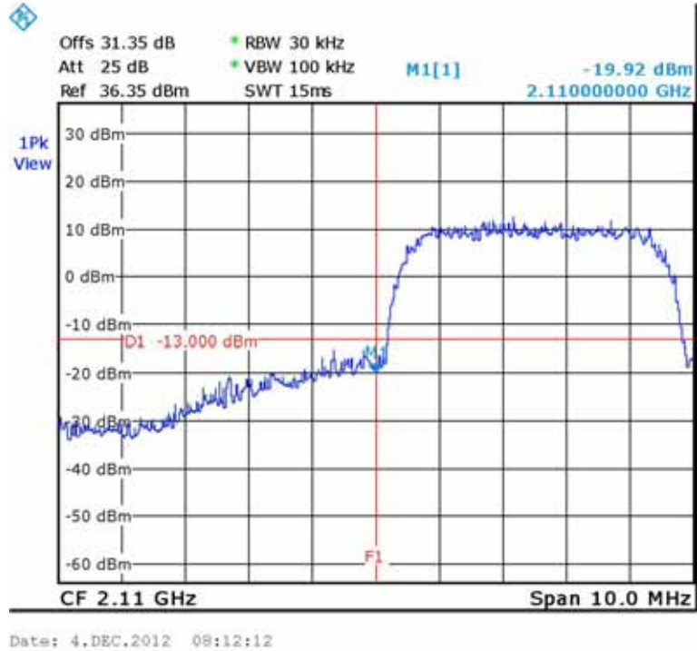
Figure 348.— W-CDMA 2112.50 MHz
