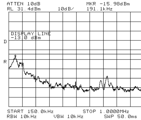
Figure 301.— 2115.00 MHz LTE
