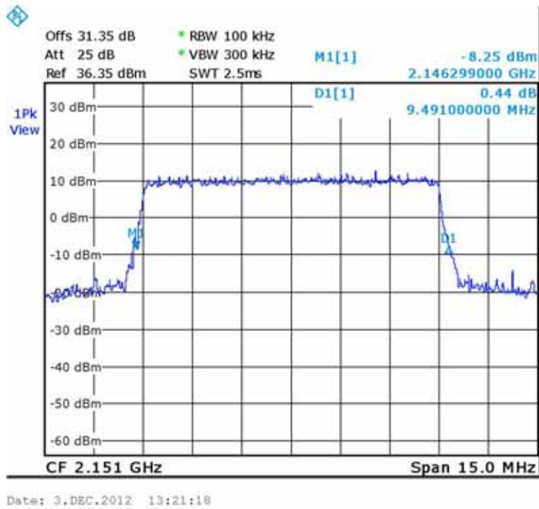
Figure 270.— LTE (2151.0 MHz) OUT
