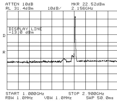
Figure 339.— 2152.50 MHz W-CDMA
