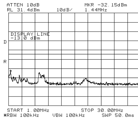
Figure 288.— 2132.50 MHz CDMA
