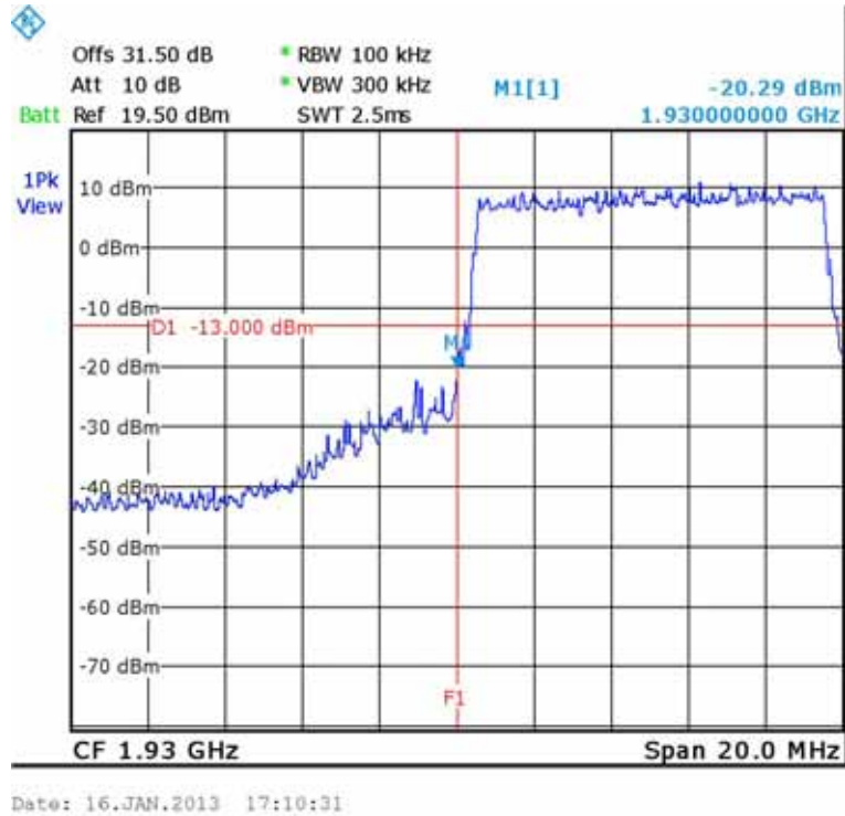
Figure 238.— 16QAM 1935.00 MHz
