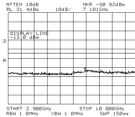
Figure 326.— 2112.50 MHz W-CDMA
