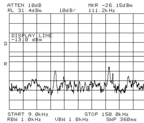
Figure 313.— 2132.50 MHz LTE
