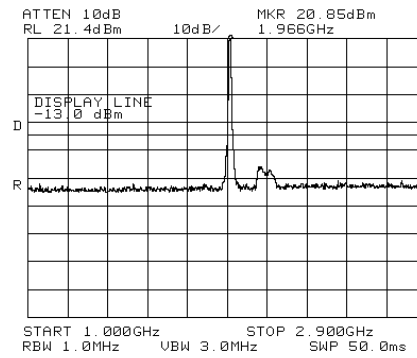
Figure 181.— 1962.50 MHz
