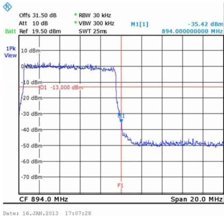
Figure 115.— QPSK 889.00 MHz
