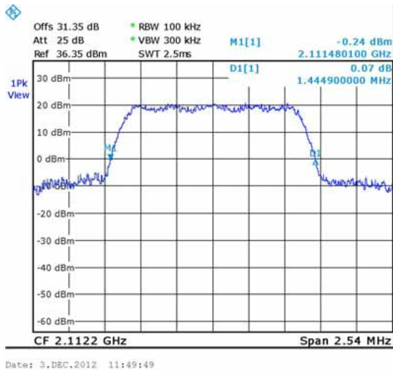
Figure 260.— CDMA (2112.2 MHz) OUT
