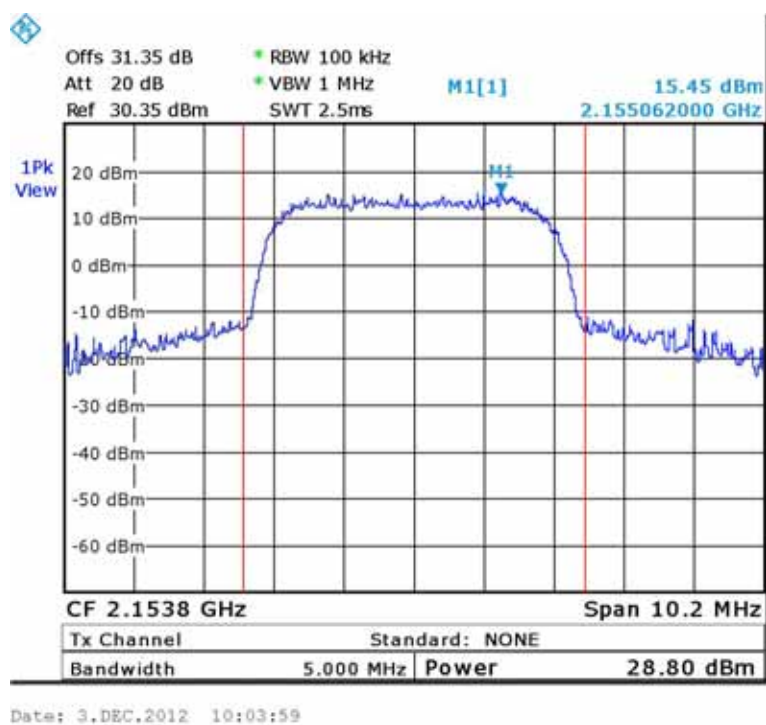
Figure 256.— W-CDMA (2153.8 MHz)
