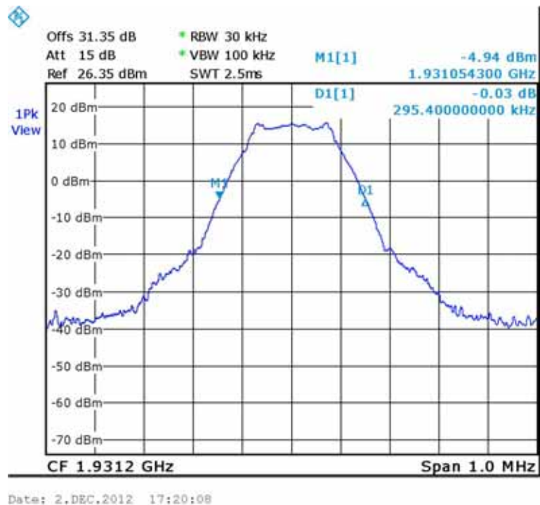
Figure 157.— Input 1931.20 MHz
