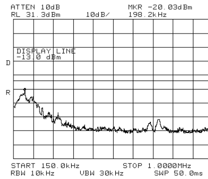
Figure 78.— 881.00 MHz
