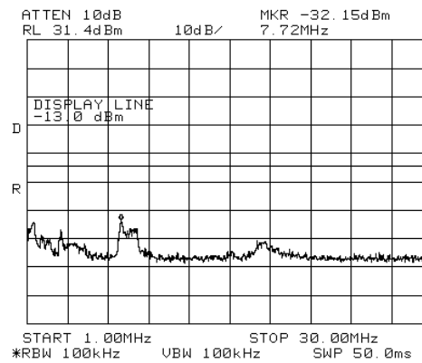
Figure 316.— 2151.00 MHz LTE
