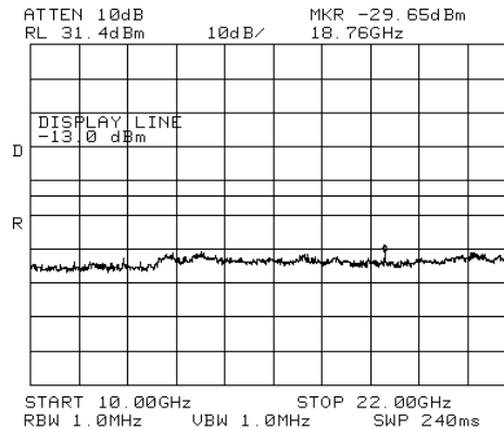
Figure 341.— 2152.50 MHz W-CDMA
