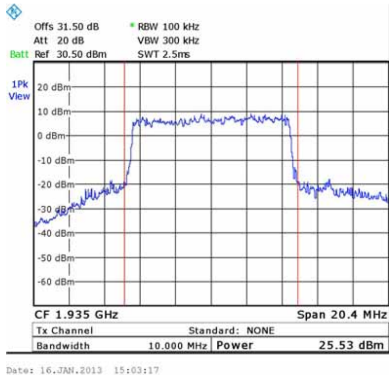
Figure 125.— 16QAM 1935.00 MHz
