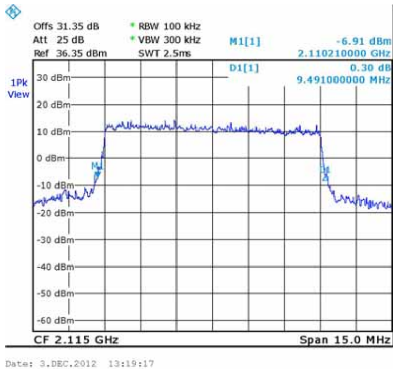
Figure 266.— LTE (2115.0 MHz) OUT
