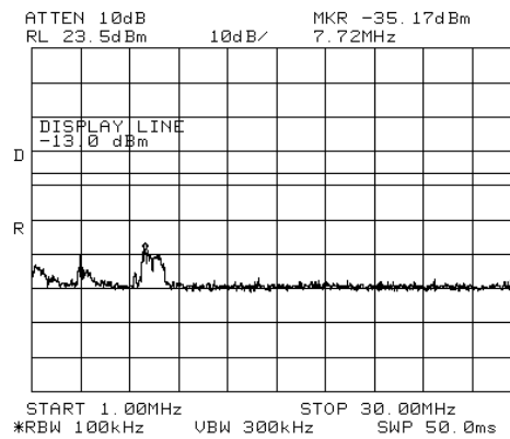
Figure 352 Intermodulation
