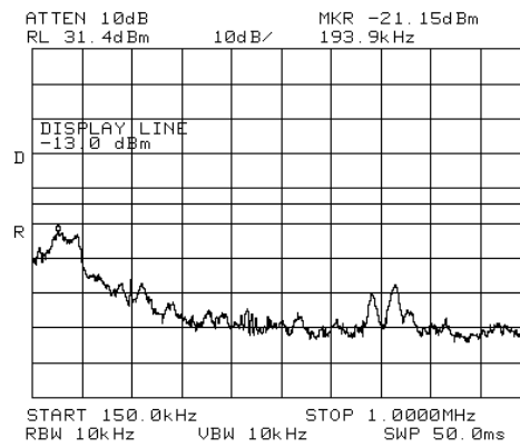
Figure 287.— 2132.50 MHz CDMA
