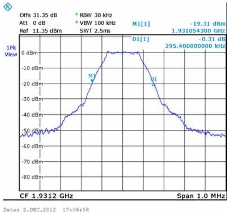
Figure 157.— Input 1931.20 MHz
