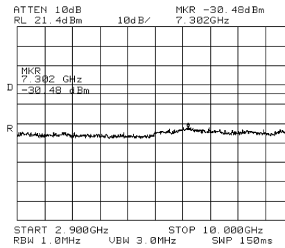
Figure 217.— 1932.50 MHz
