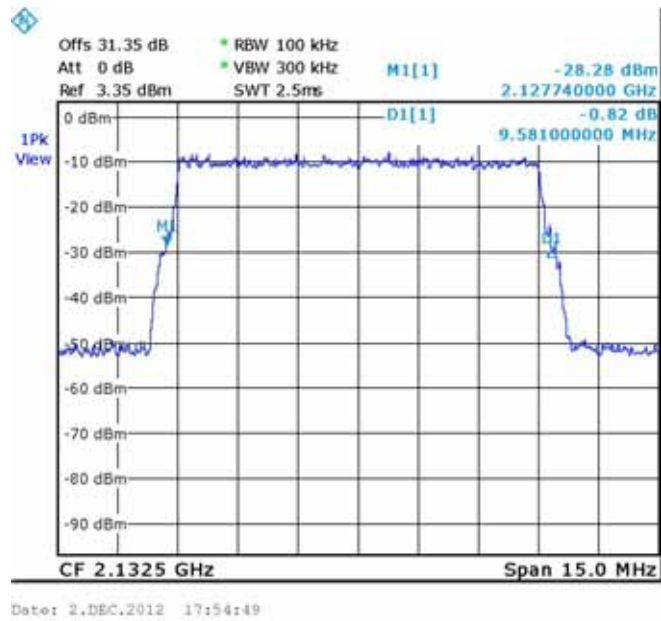
Figure 267.— LTE (2132.5 MHz) IN
