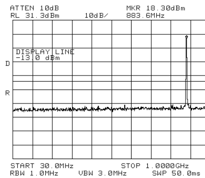
Figure 80.— 881.00 MHz
