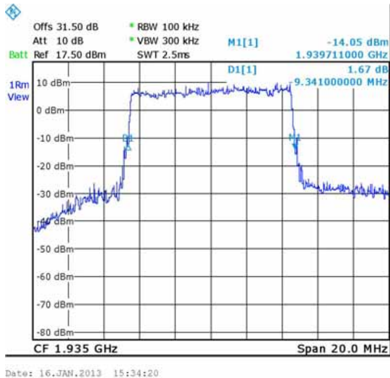
Figure 145.— 16QAM Input 1935.00 MHz
