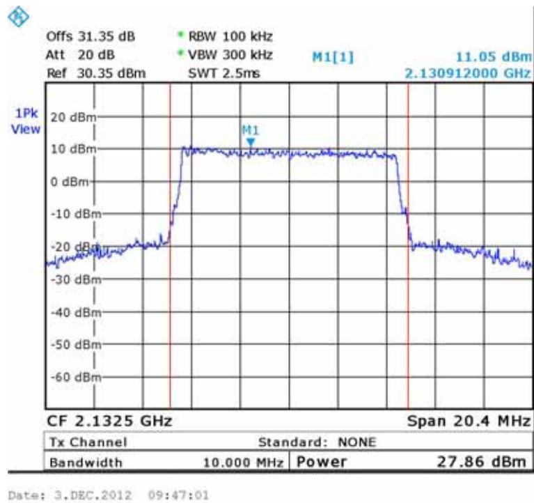
Figure 252.— LTE (2132.5 MHz)
