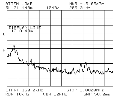
Figure 315.— 2151.00 MHz LTE
