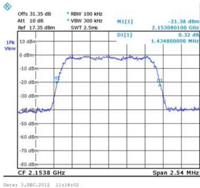
Figure 263.— CDMA (2153.8 MHz) IN
