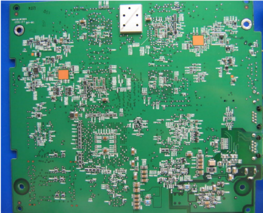
Photograph No.7 PCB second side view
