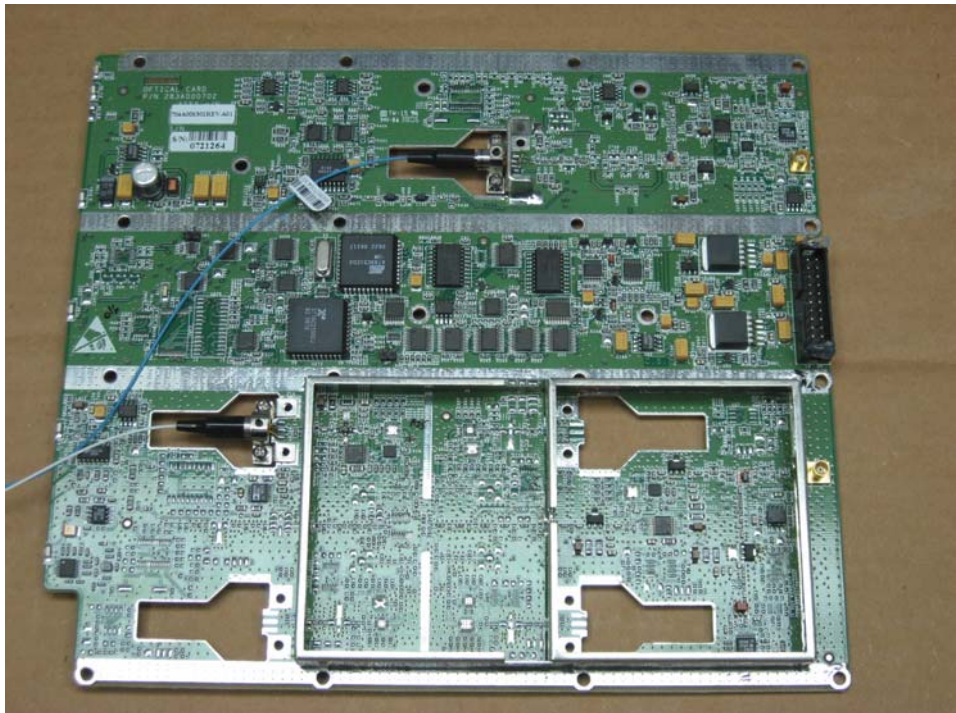
1500-UHF-BU-2 Optical Card Side 1
