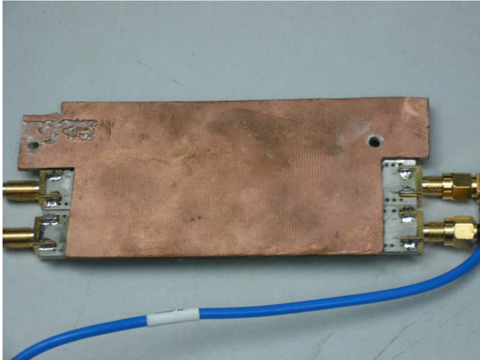
1500-UHF-BU-2 Filter Side 2
