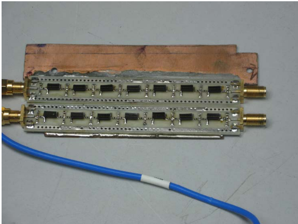
1500-UHF-BU-2 Filter Side 1
