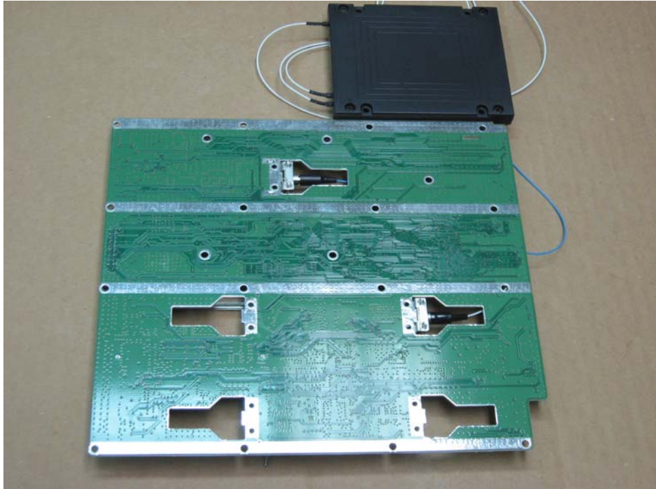
1500-UHF-RU Optical card With Laser Side 2
