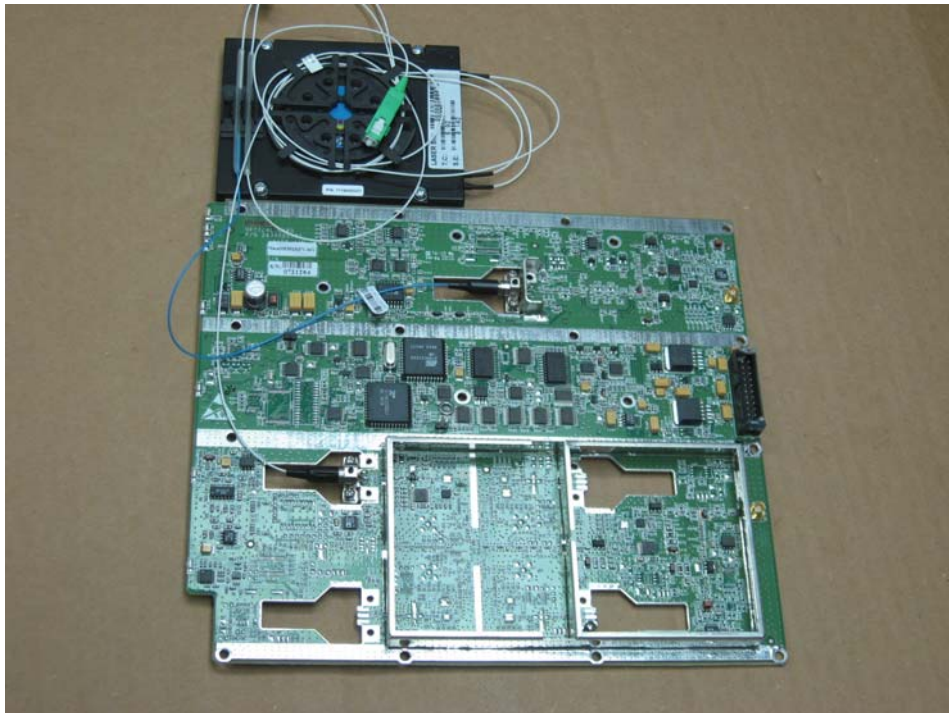
1500-UHF-BU-2 Optical card With Laser Side 1
