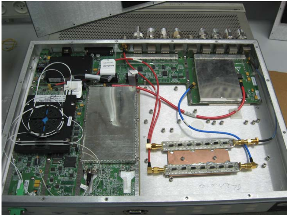
1500-UHF-RU PCB's In Case
