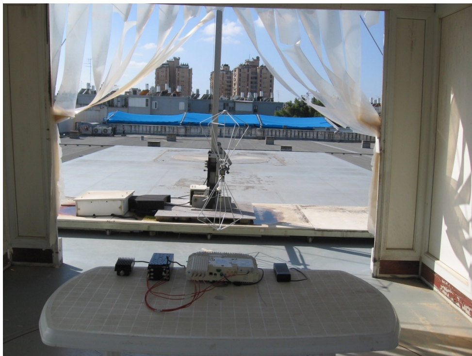
Figure 3. Radiated Emission Test 30 - 200 MHz
