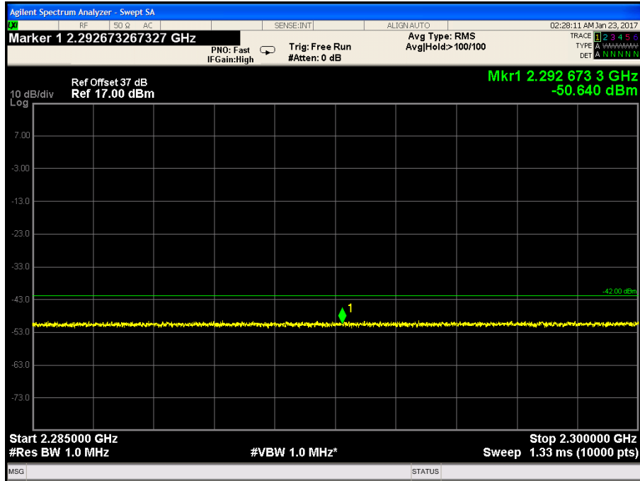
Figure 48 — 2285.0 MHz-2300.0MHz - 16QAM
