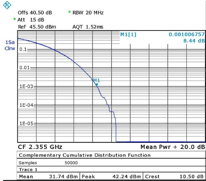
Figure 23. —64QAM, 2355.0 MHz
