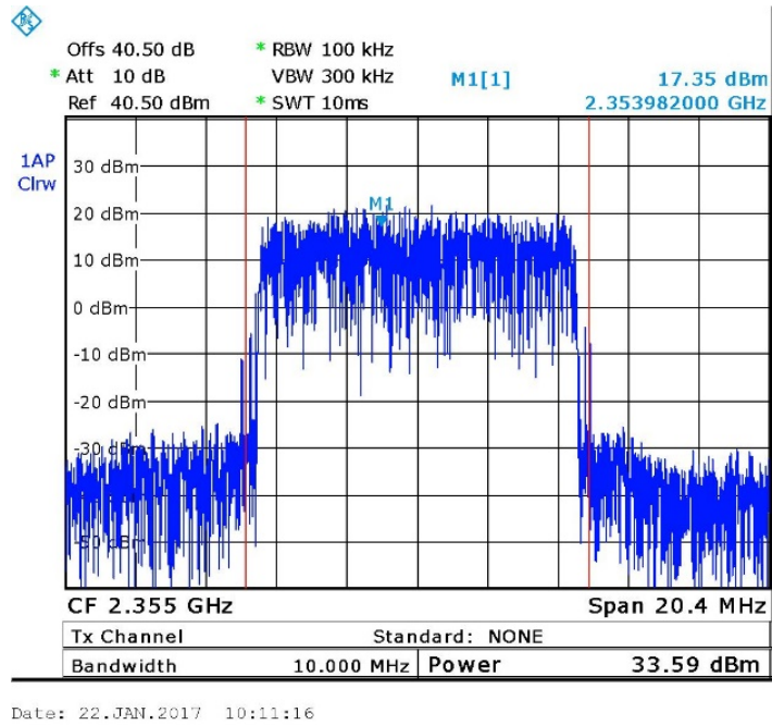
Figure 12. — 2355.0 MHz –64QAM
