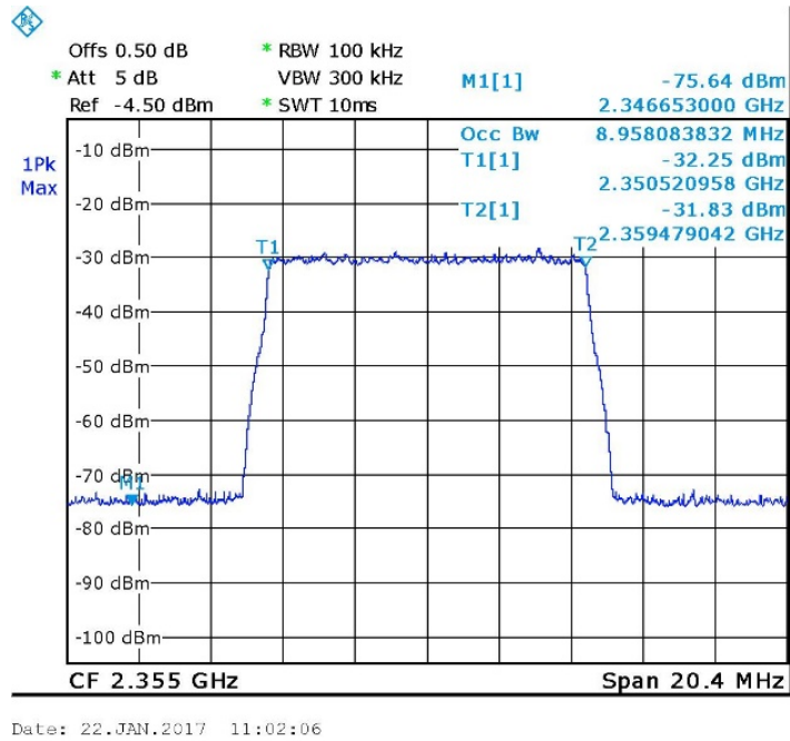
Figure 30 Occupied Bandwidth INPUT, 16QAM
