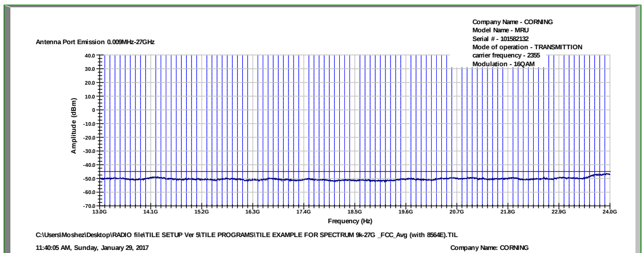
Figure 57. —13,000.0 MHz-24,000MHz - 16QAM
