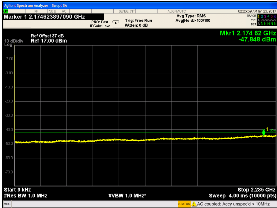
Figure 36. — 0.009 MHz-2285.0MHz –64QAM
