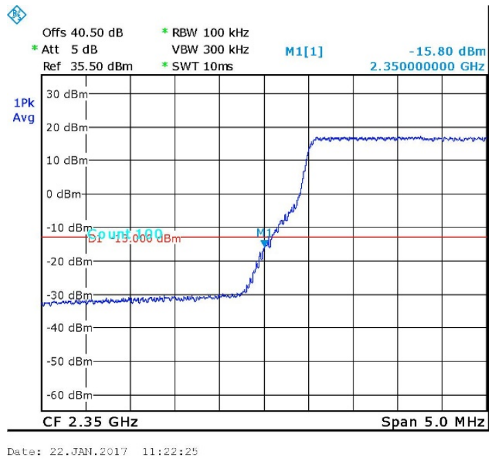
Figure 71. — Lower Block Edge -1MHz -64QAM
