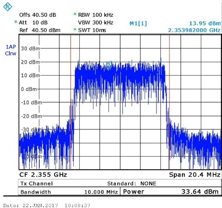
Figure 14. — 2355.0 MHz QPSK
