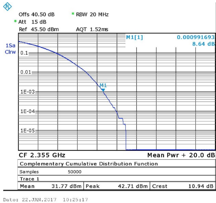
Figure 25. — QPSK, 2355.0 MHz
