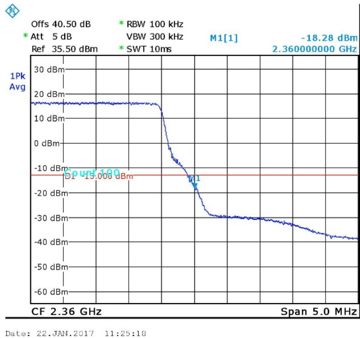
Figure 76. — Upper Band Edge +1MHz – QPSK
