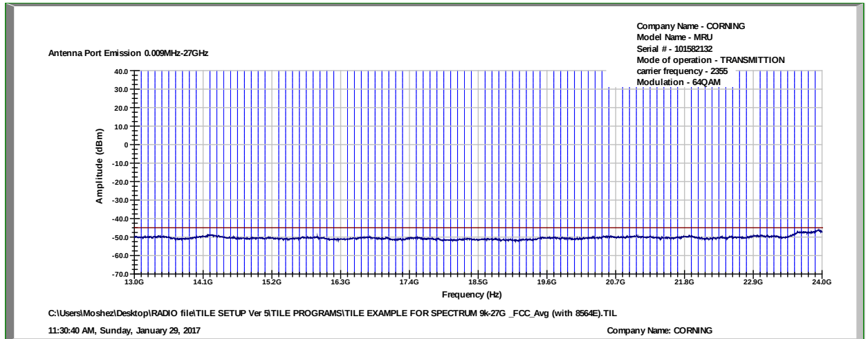
Figure 46. —13,000.0 MHz-24,000MHz –64QAM
