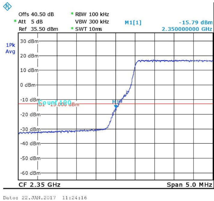
Figure 75. — Lower Block Edge -1MHz – QPSK
