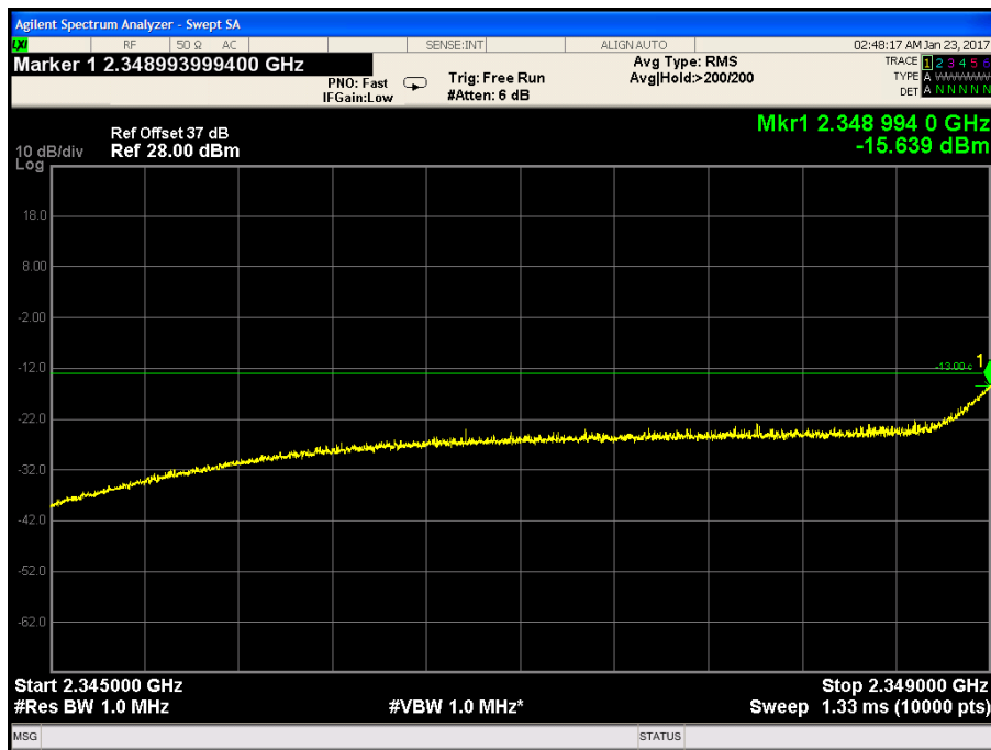
Figure 63. — 2345.0 MHz-2349.0MHz – QPSK
