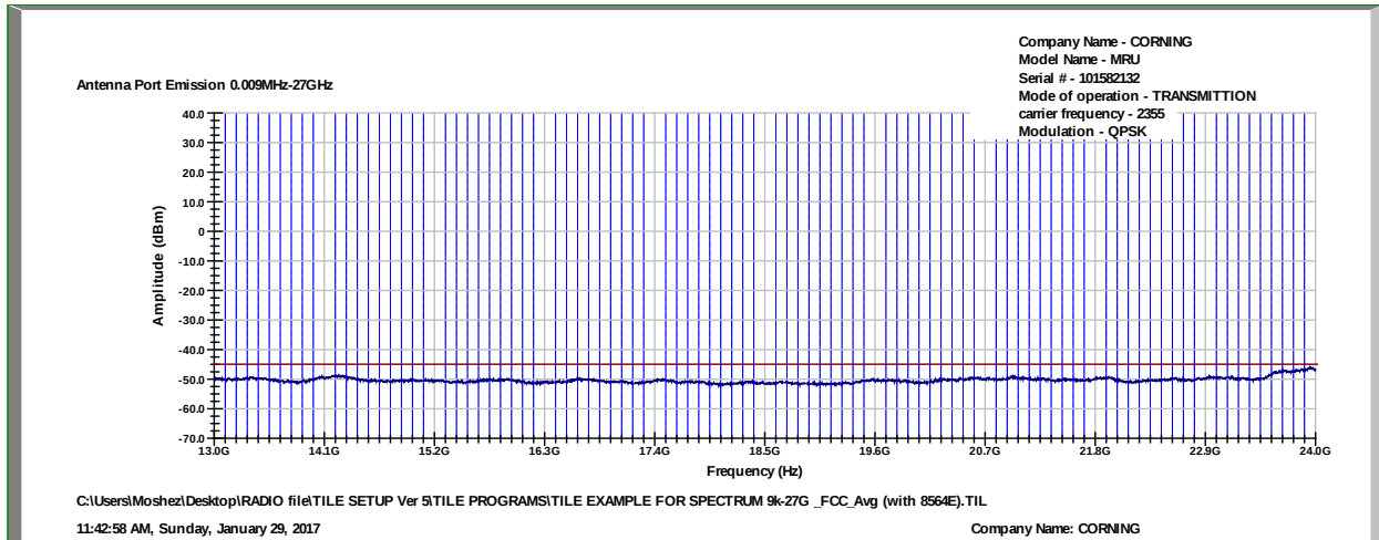
Figure 68. —13,000.0 MHz-24,000MHz – QPSK
