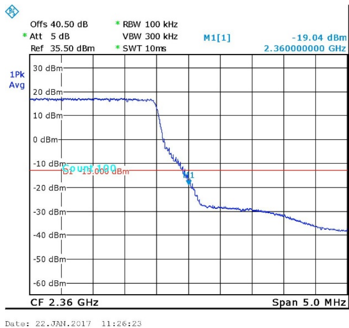
Figure 72. — Upper Band Edge +1MHz -64QAM
