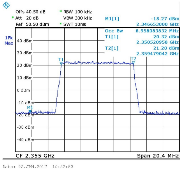
Figure 31 Occupied Bandwidth OUTPUT, 16QAM
