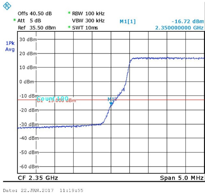
Figure 73. — Lower Block Edge -1MH – 16QAM
