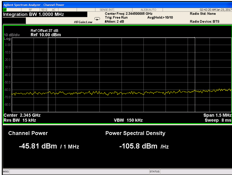
Figure 62. — 2344.0 MHz-2345MHz – QPSK
