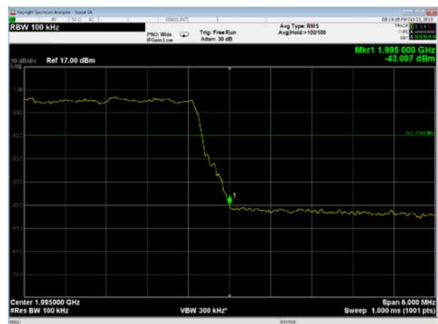
Figure 166 10MHz BW, 1990MHz
