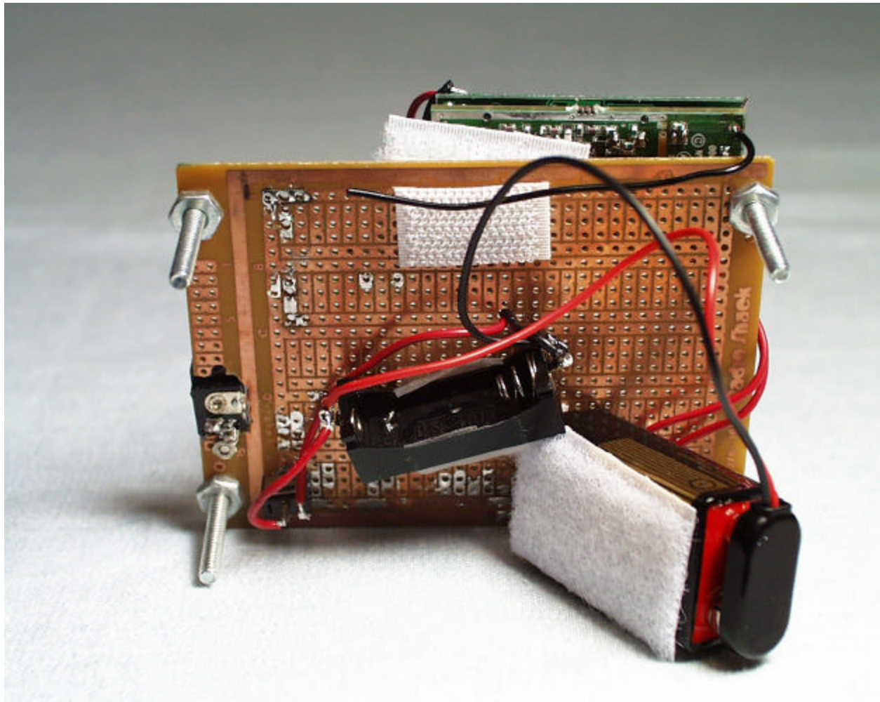
Back view of the test jig used to test the transmitter
