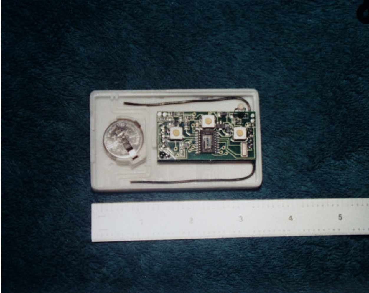
Inside view of the 6000-4
