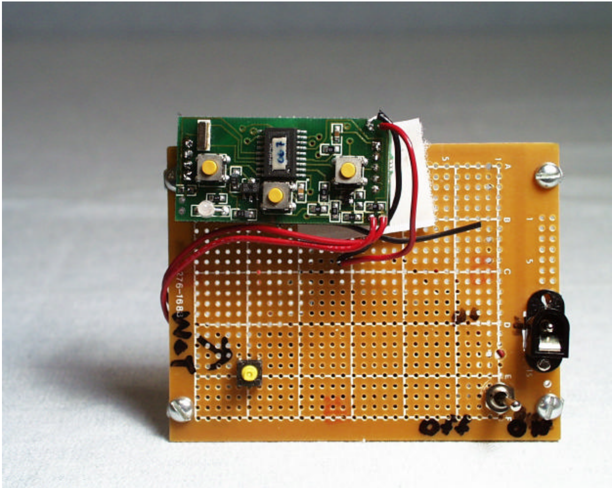
Front view of the test jig used to test the transmitter
