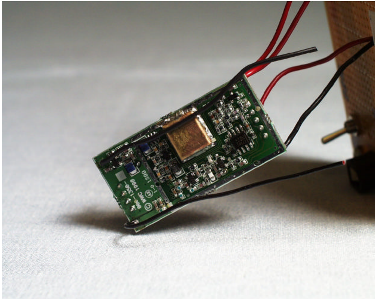
Back view of the transmitter and interface boards
