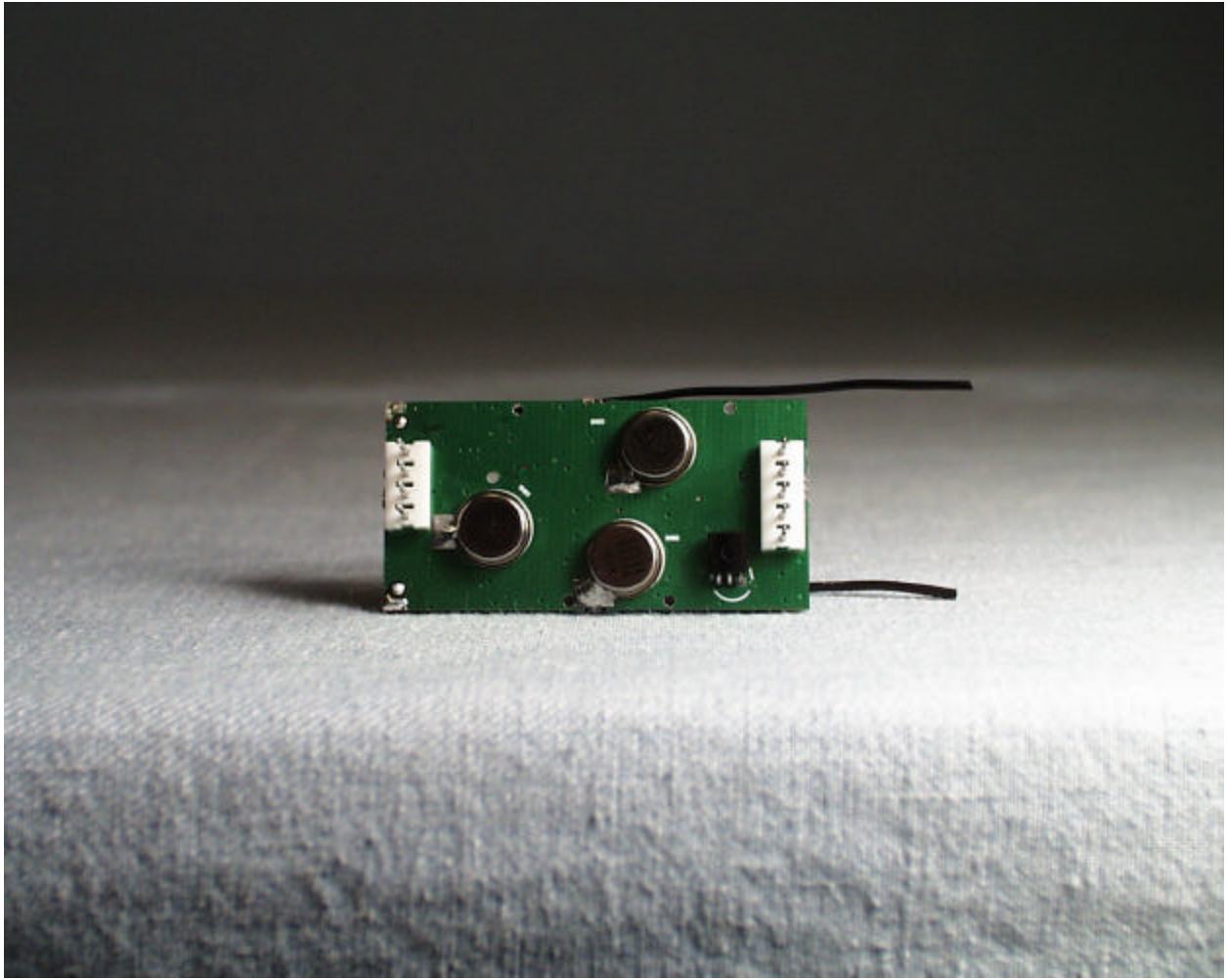
Back view of the transmitter board
