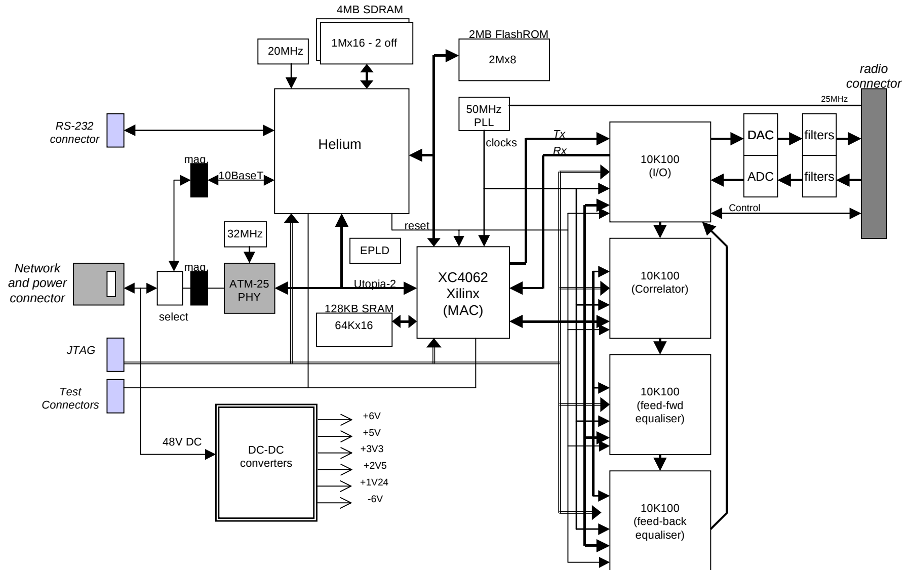
Figure 2 : System Motherboard.
