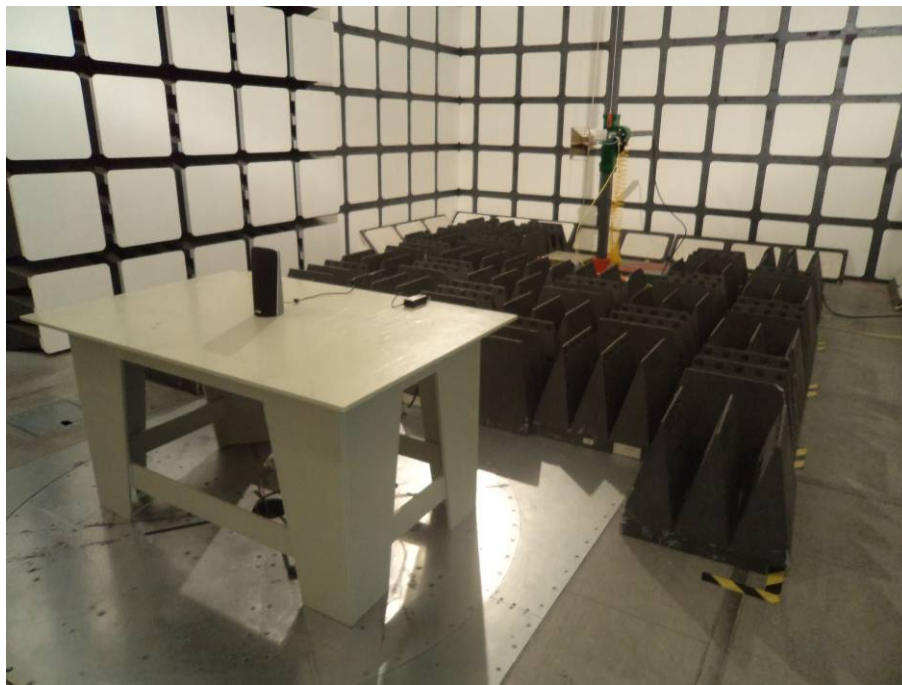
Above 1 GHz: Spurious Radiated Emissions - Front View
