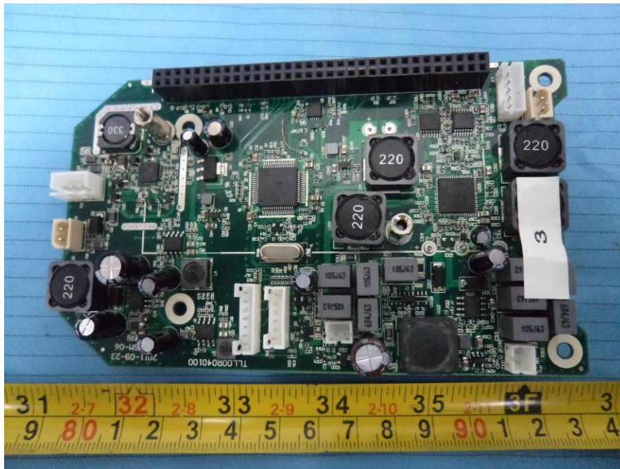
EUT – Main Board without RF Module Top View
