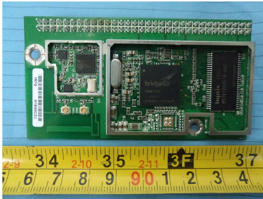
EUT – RF Module Shielding off Top View
