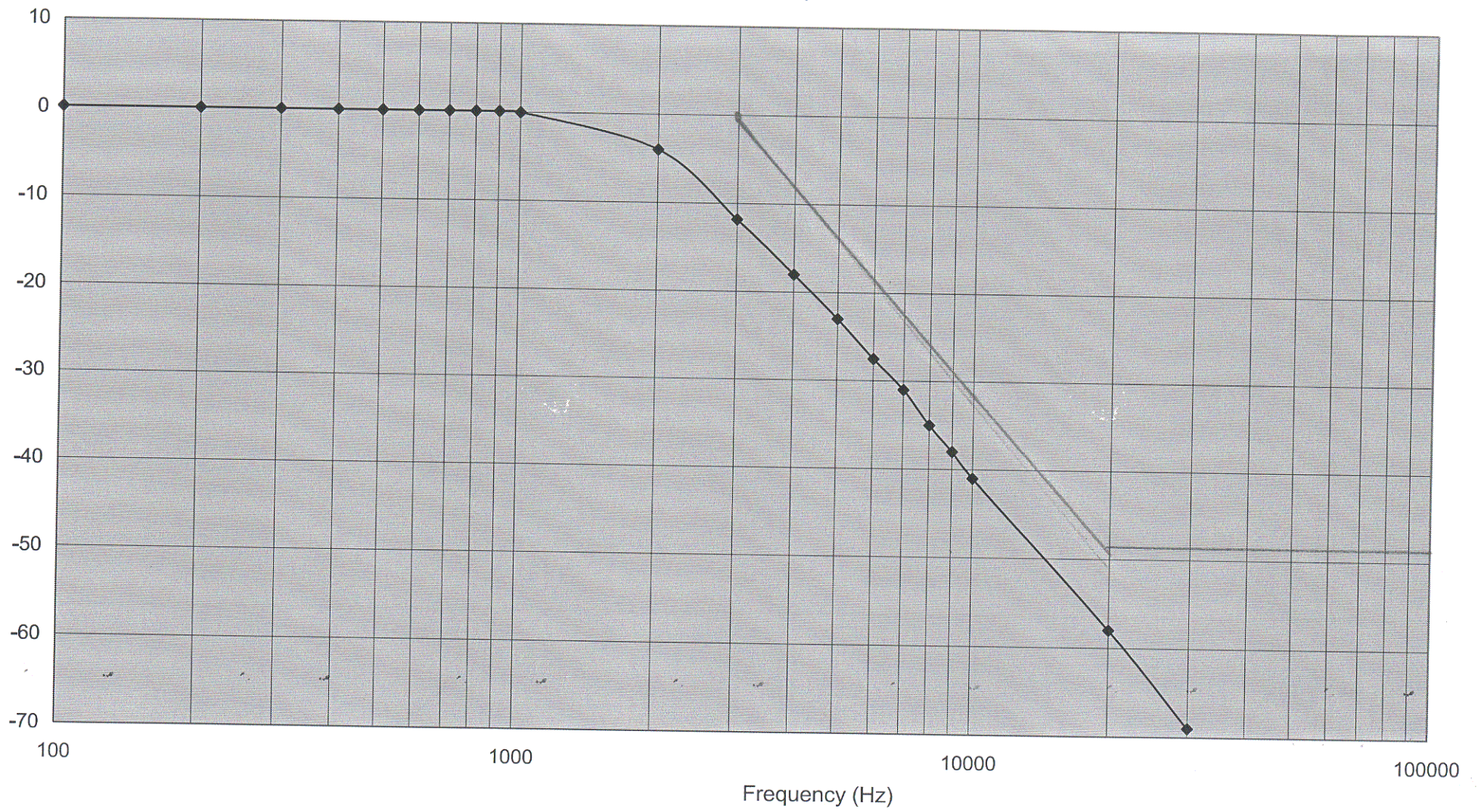
FRS Model No. VC968 Frequency response of audio post limiter filter
