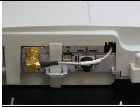
Figure 15 – internal (service) antenna cable, manual power selector, and auxiliary jack on the left side
