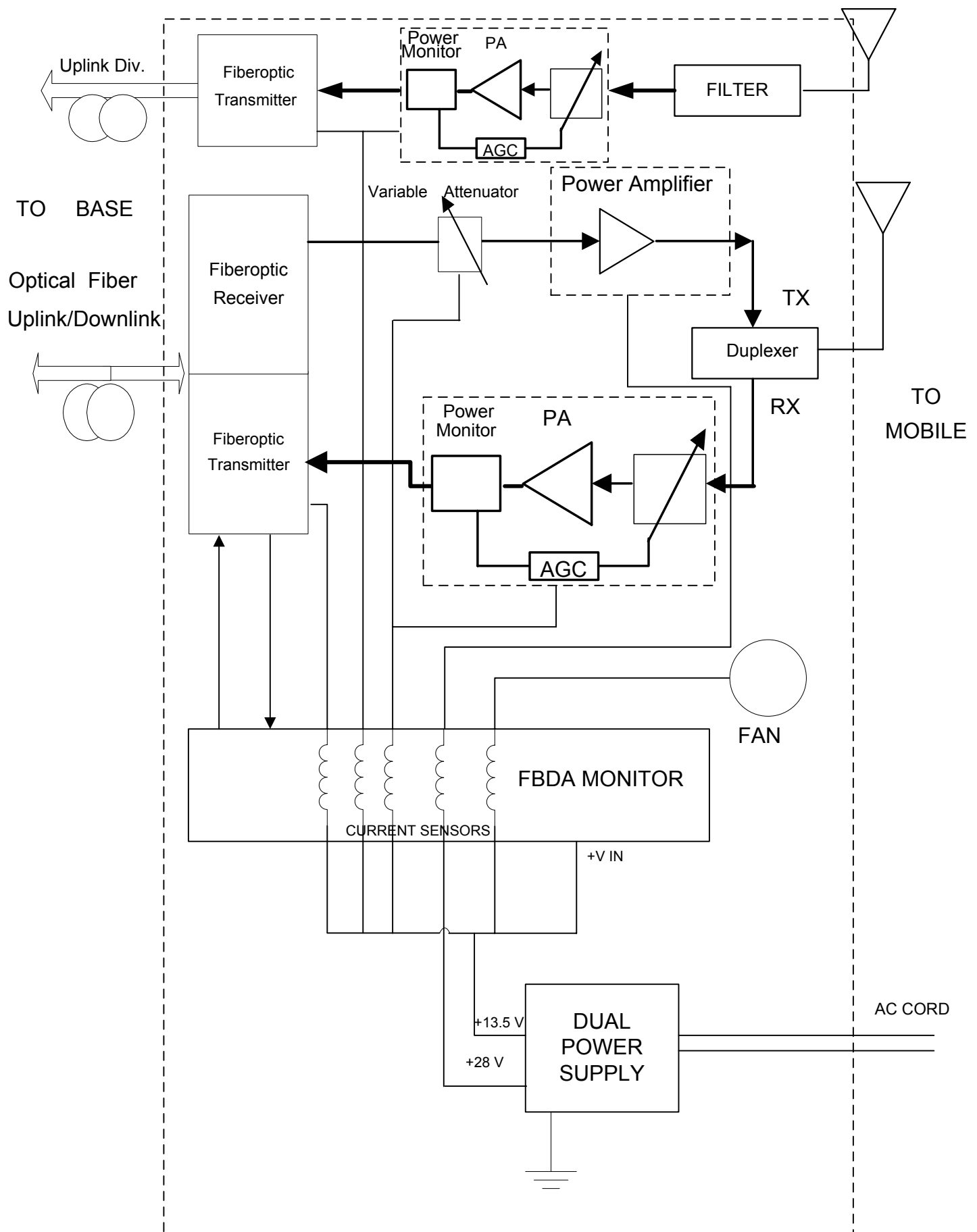
FBDA-SMR8-50W-DIV ELEELECTRICAL SCHEMATICS
