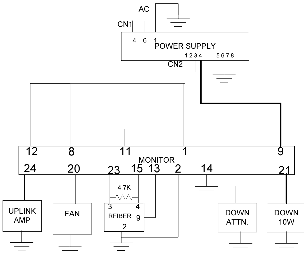
FBDA PCS 10 W WIRING DIAGRAM
