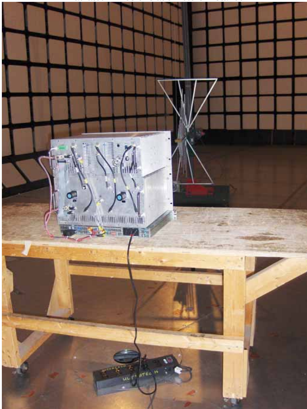
Radiated Emissions at 3 Meters Distance
