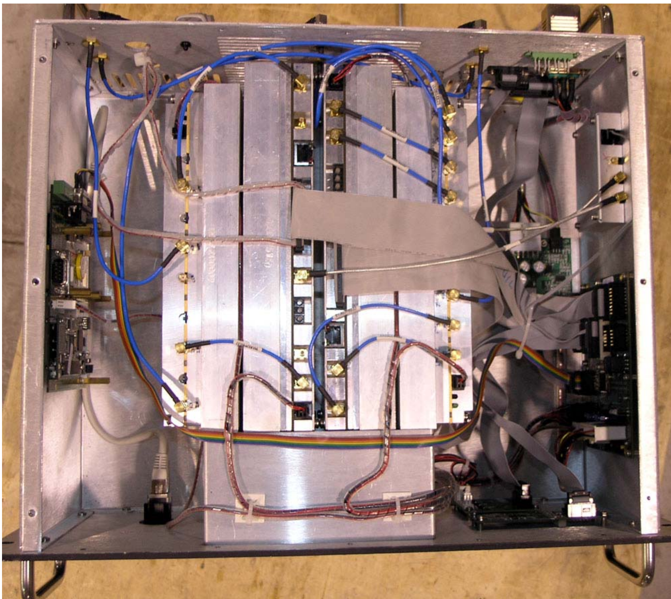
Dekolink Wireless Ltd. Dual Band Bi-Directional Amplifier, Model MW-DCSB-40D95-700/800-24-AC-R FCC ID: OIWDCSB40D95AC, IC: 4589A-DCSB4090
