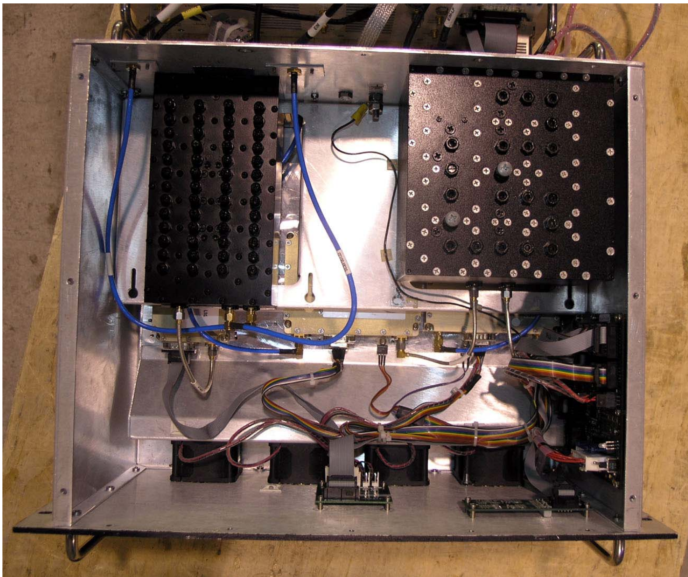
Dekolink Wireless Ltd. Dual Band Bi-Directional Amplifier, Model MW-DCSB-40D95-700/800-24-AC-R FCC ID: OIWDCSB40D95AC, IC: 4589A-DCSB4090
