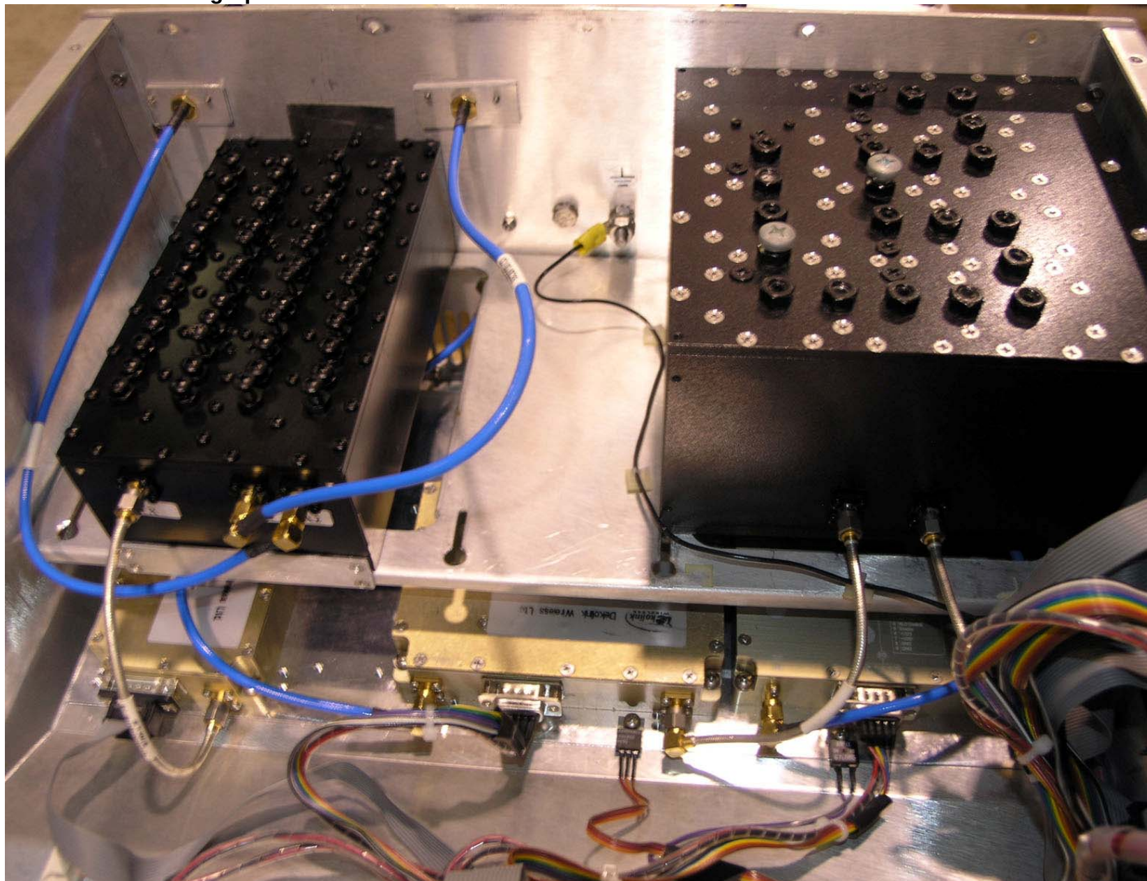
Dekolink Wireless Ltd. Dual Band Bi-Directional Amplifier, Model MW-DCSB-40D95-700/800-24-AC-R FCC ID: OIWDCSB40D95AC, IC: 4589A-DCSB4090
