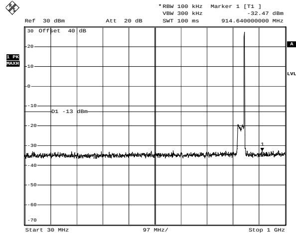
Uplink - CDMA - High Channel Date: 23.NOV.2006 00:10:10
