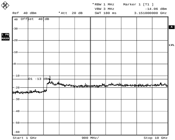
Downlink - GSM - High Channel Date: 22.NOV.2006 21:57:16
