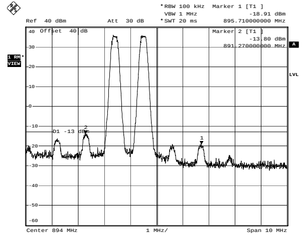
Downlink - GSM - 3rd Order Intermodulation Date: 22.NOV.2006 22:09:55
