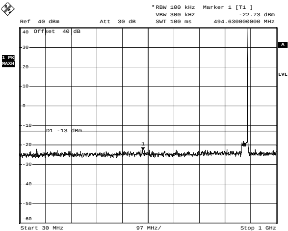
Downlink - GSM - High Channel Date: 22.NOV.2006 21:57:57
