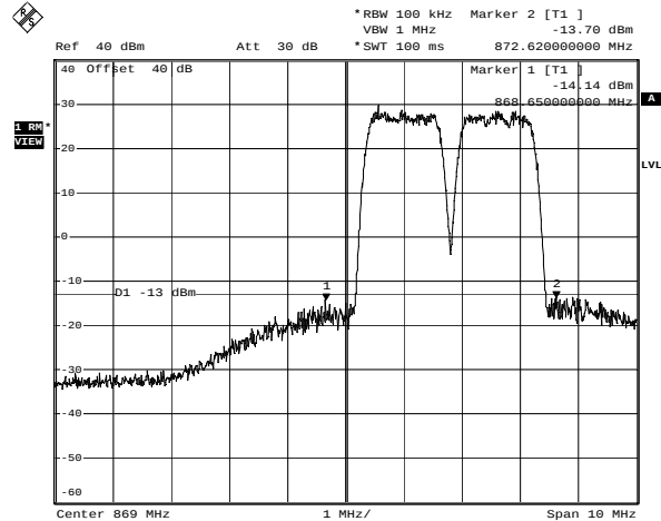
Downlink - CDMA - 3rd Order Intermodulation Date: 23.NOV.2006 23:38:08
