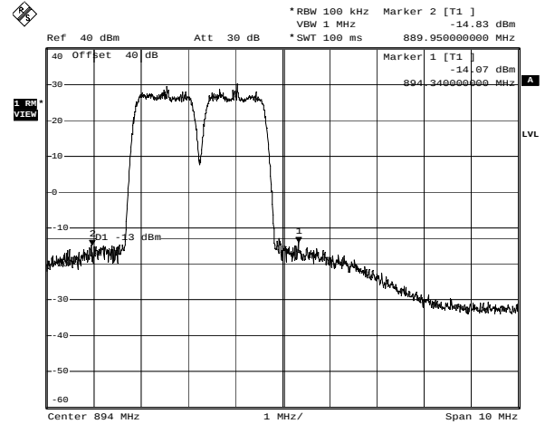
Downlink - CDMA - 3rd Order Intermodulation Date: 22.NOV.2006 22:12:49
