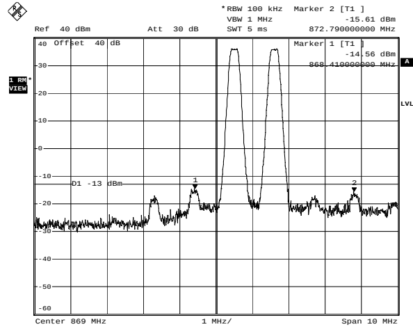
Downlink - GSM - 3rd Order Intermodulation Date: 22.NOV.2006 22:07:09
