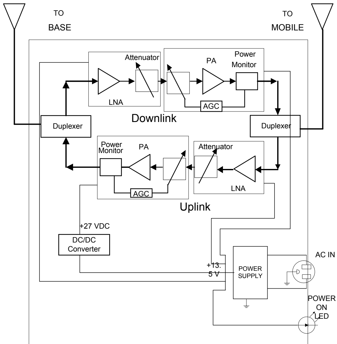
CBDA-10W80 ELECTRICAL SCHEMATICS
